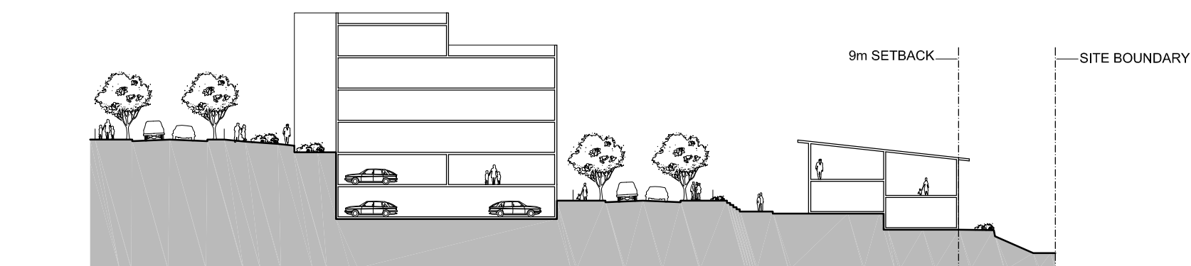
Section B-B
