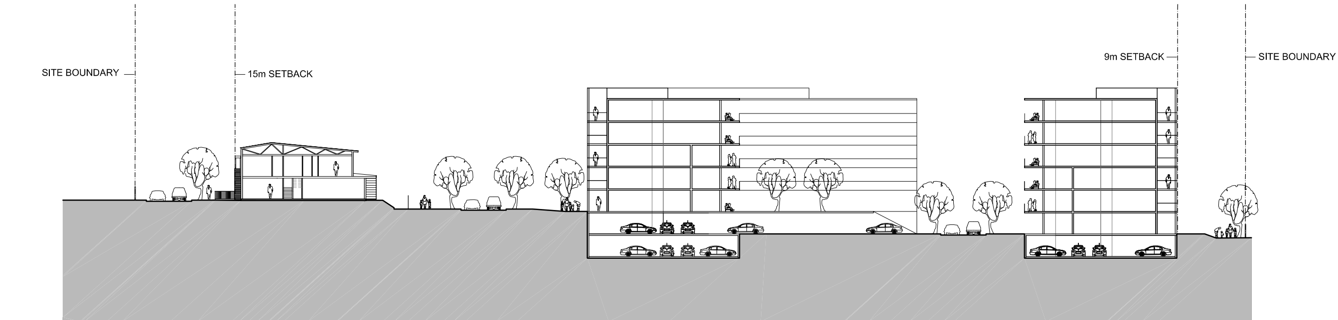
Section F-F
