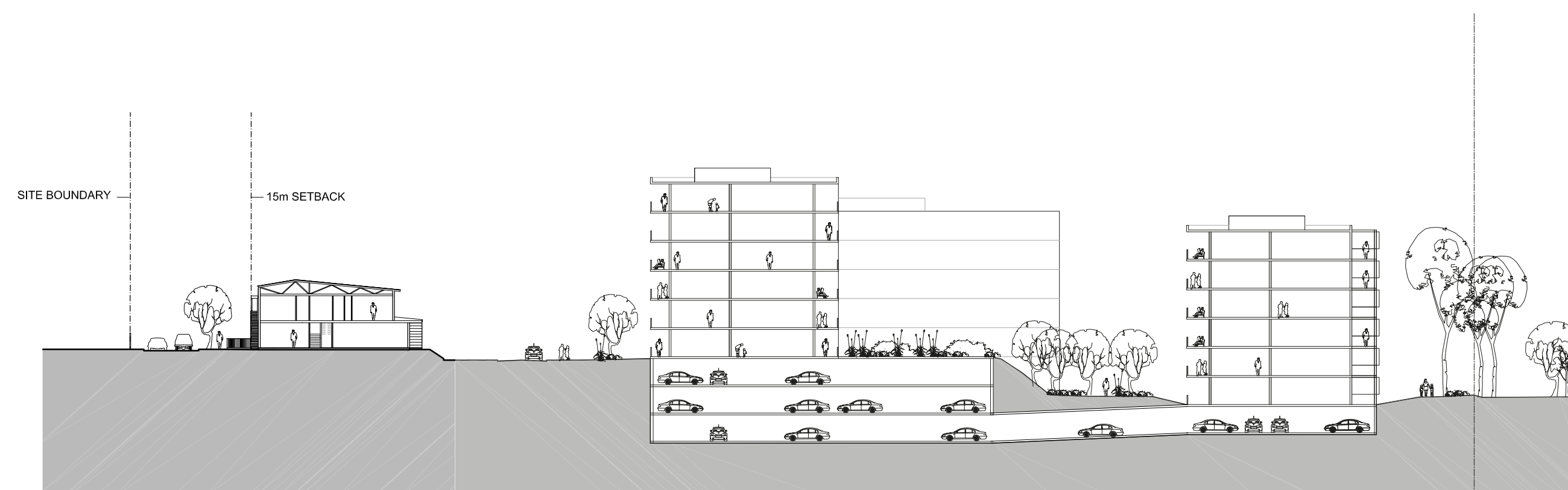
Section F-F
