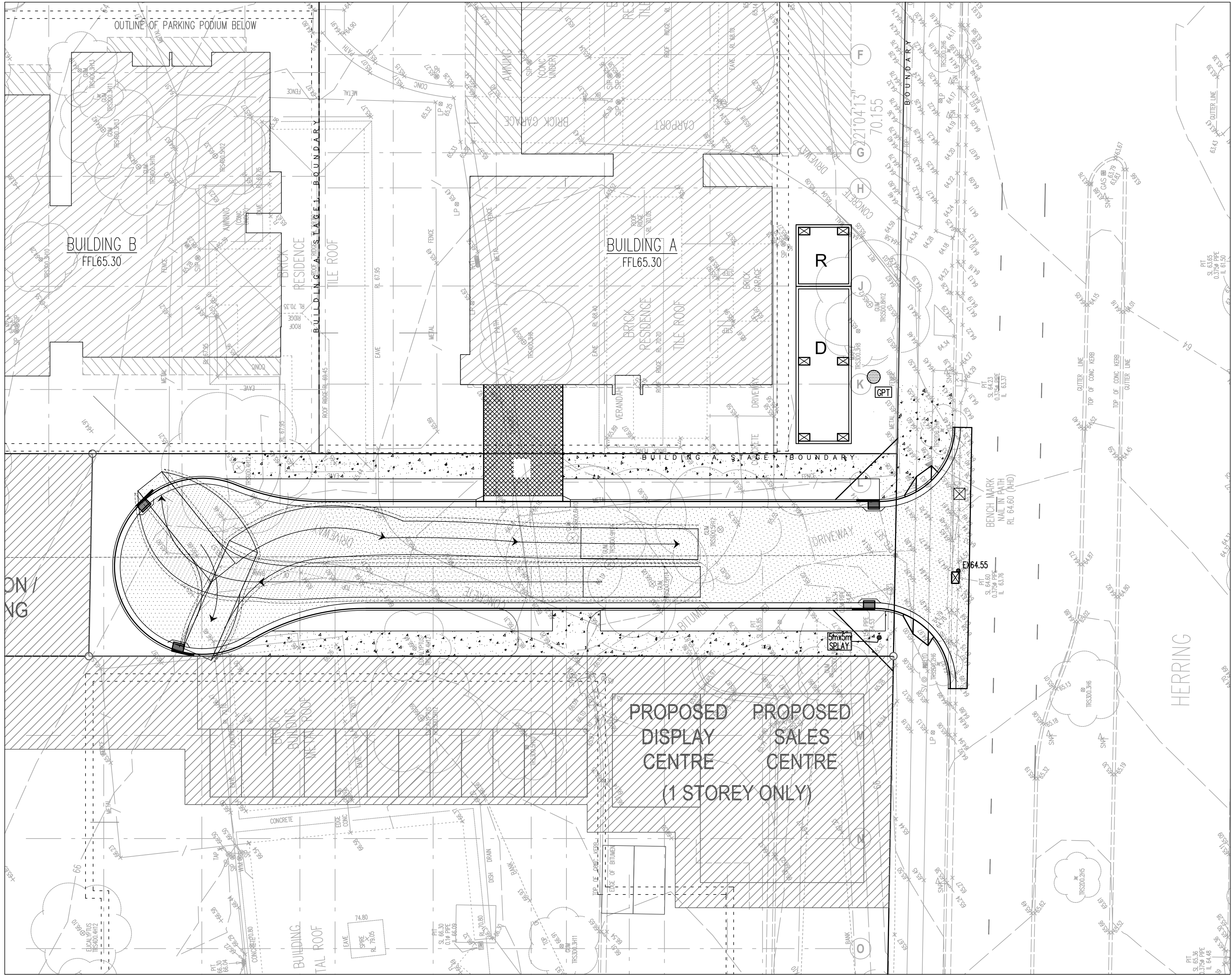
9.30m RYDE GARBAGE TRUCK
