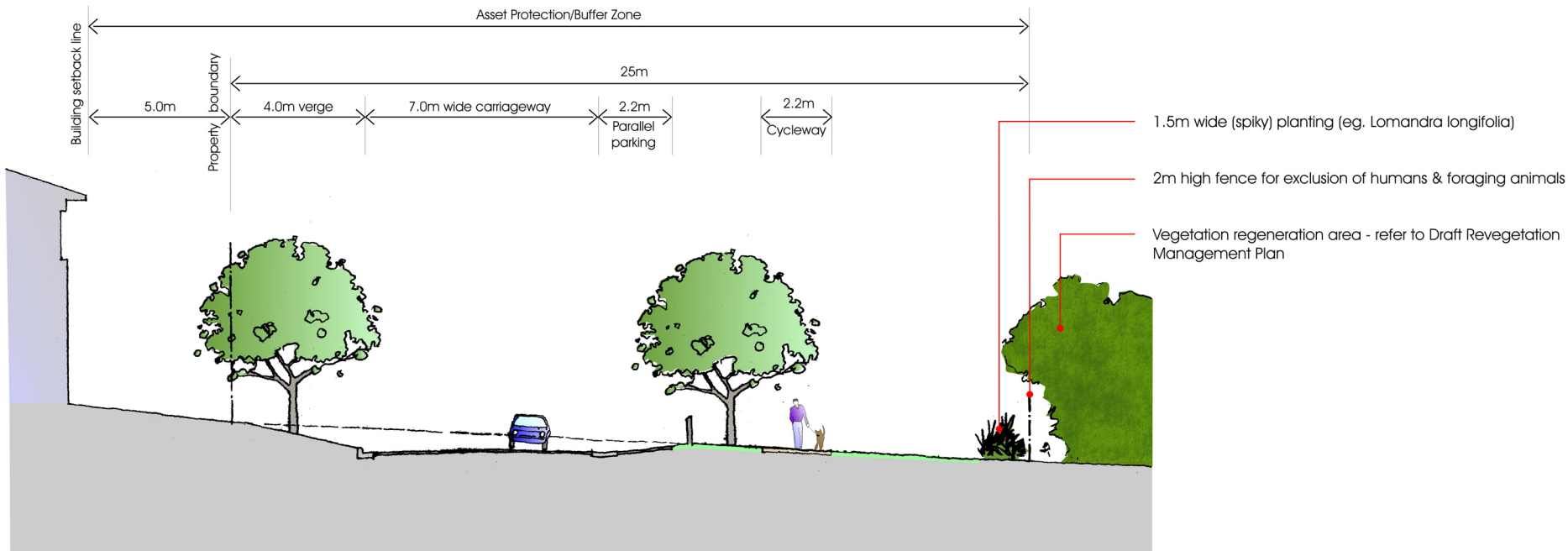
Typical Cross Section AA Scale 1:100 @ A1
