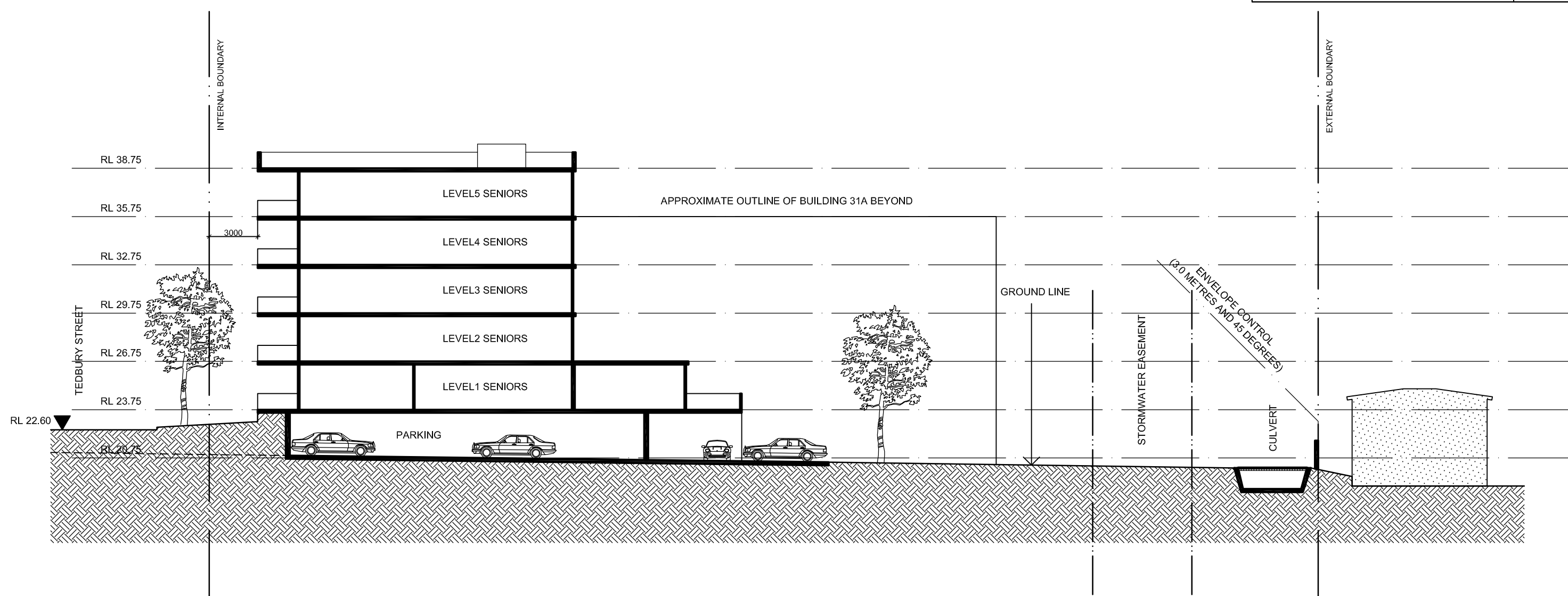
SECTION DD LOT 31 SENIORS LIVING COMPLEX
