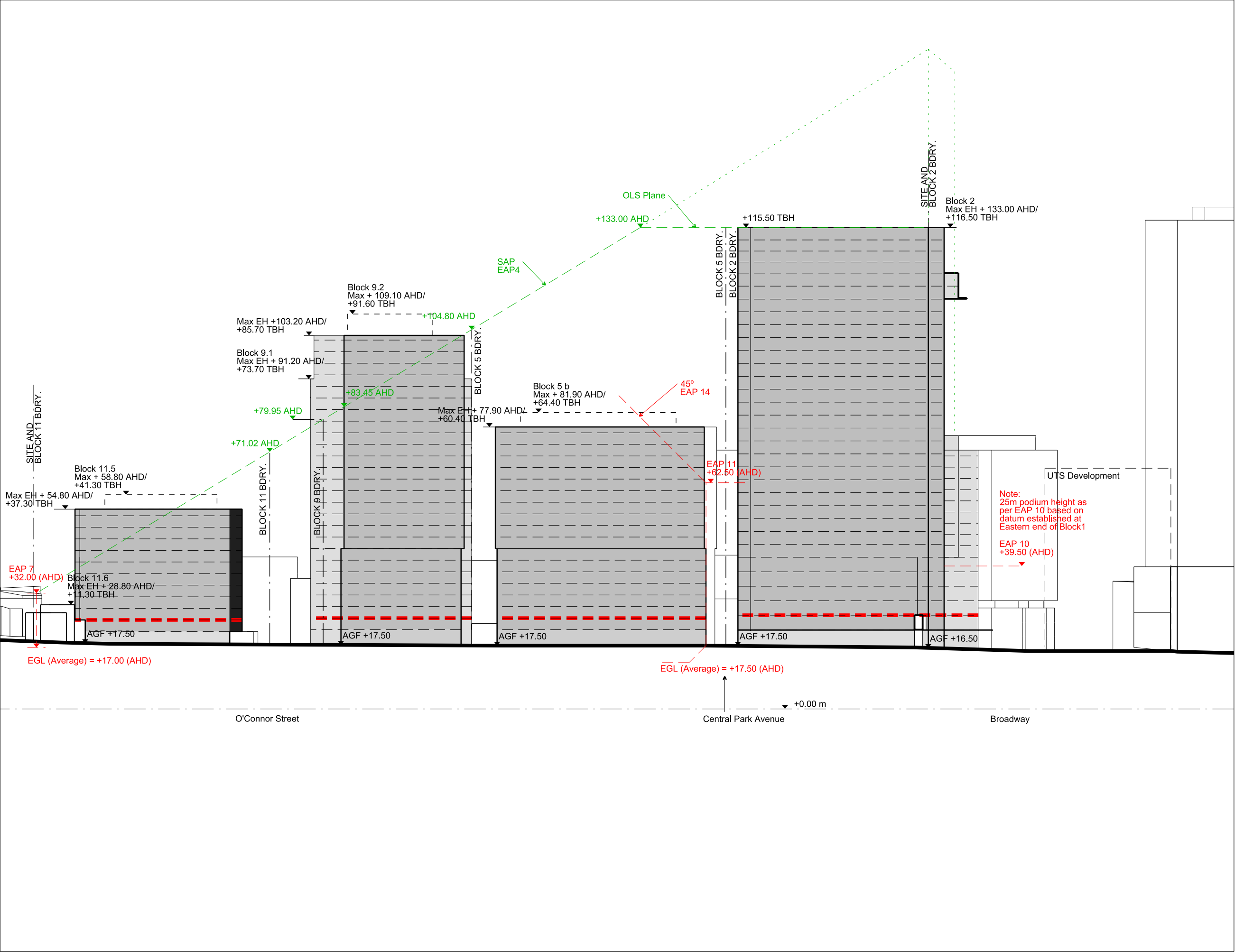
01 East Elevation 1:1000
