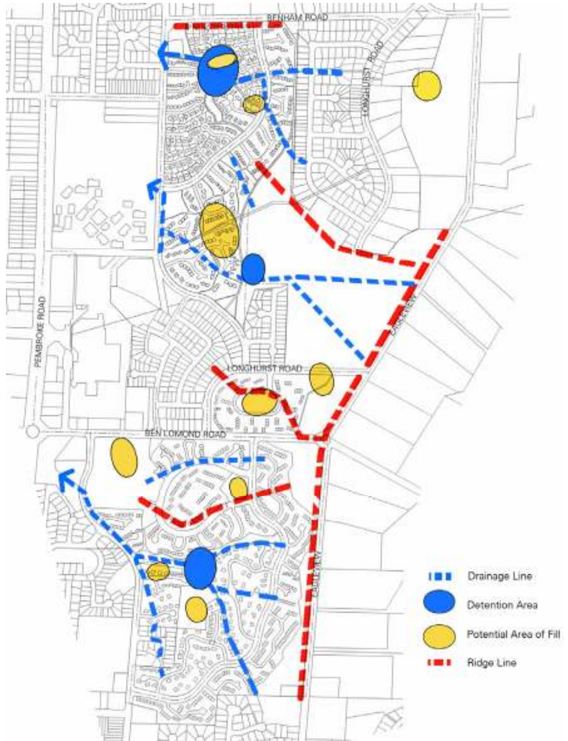
Figure 9. Drainage and Fill
