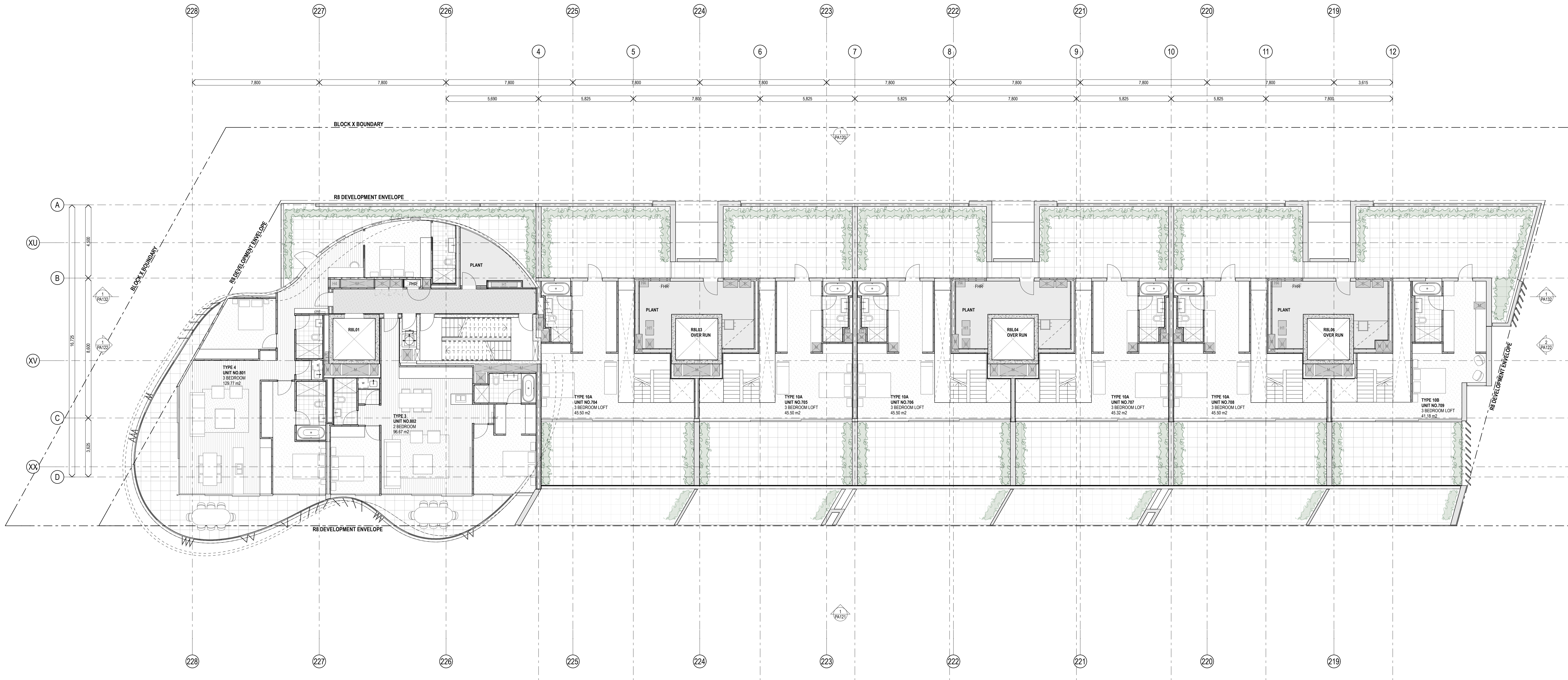
1 PLAN Level 8 1:100
