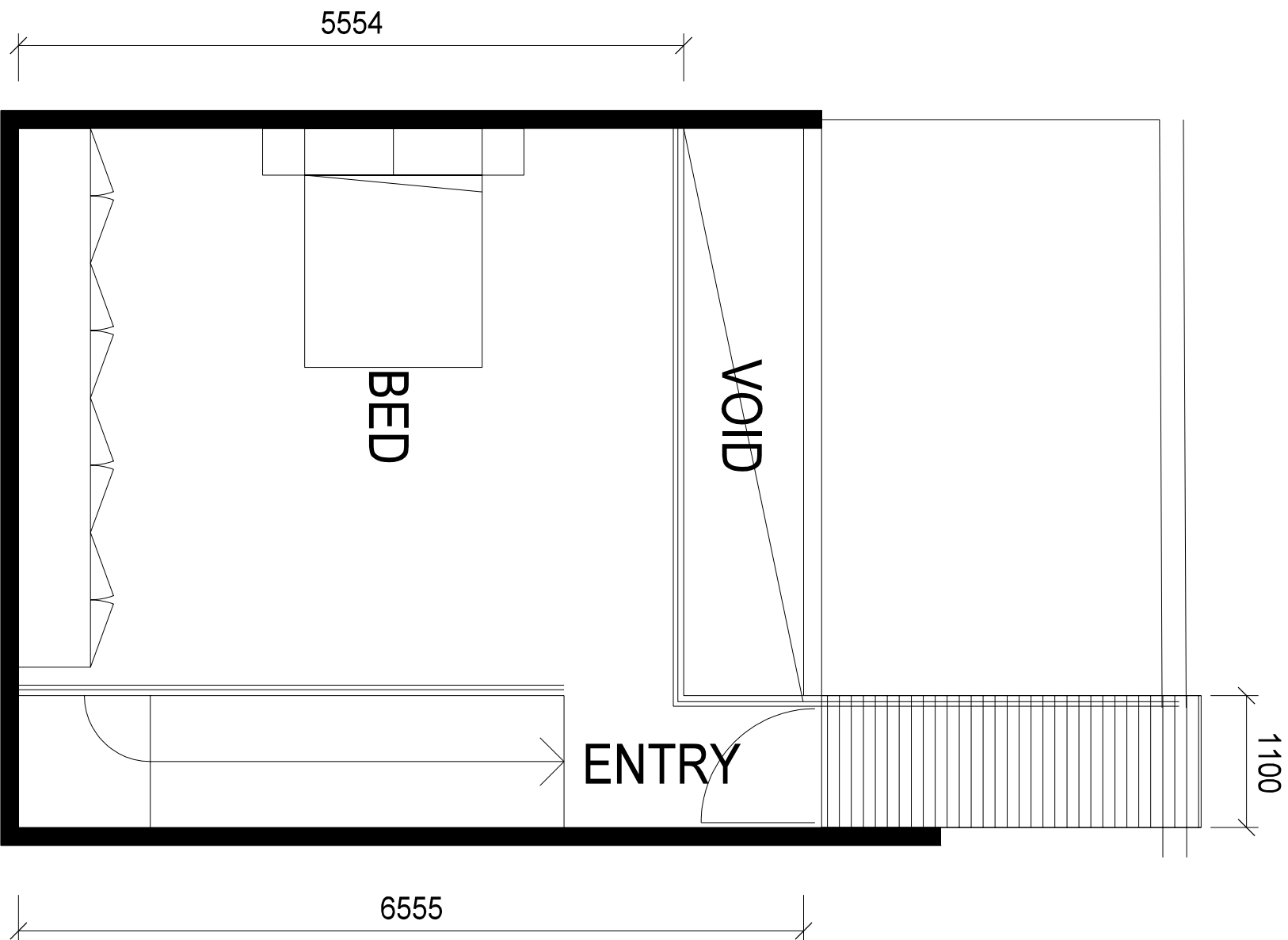
APARTMENT TYPE 'C' UPPER LEVEL
