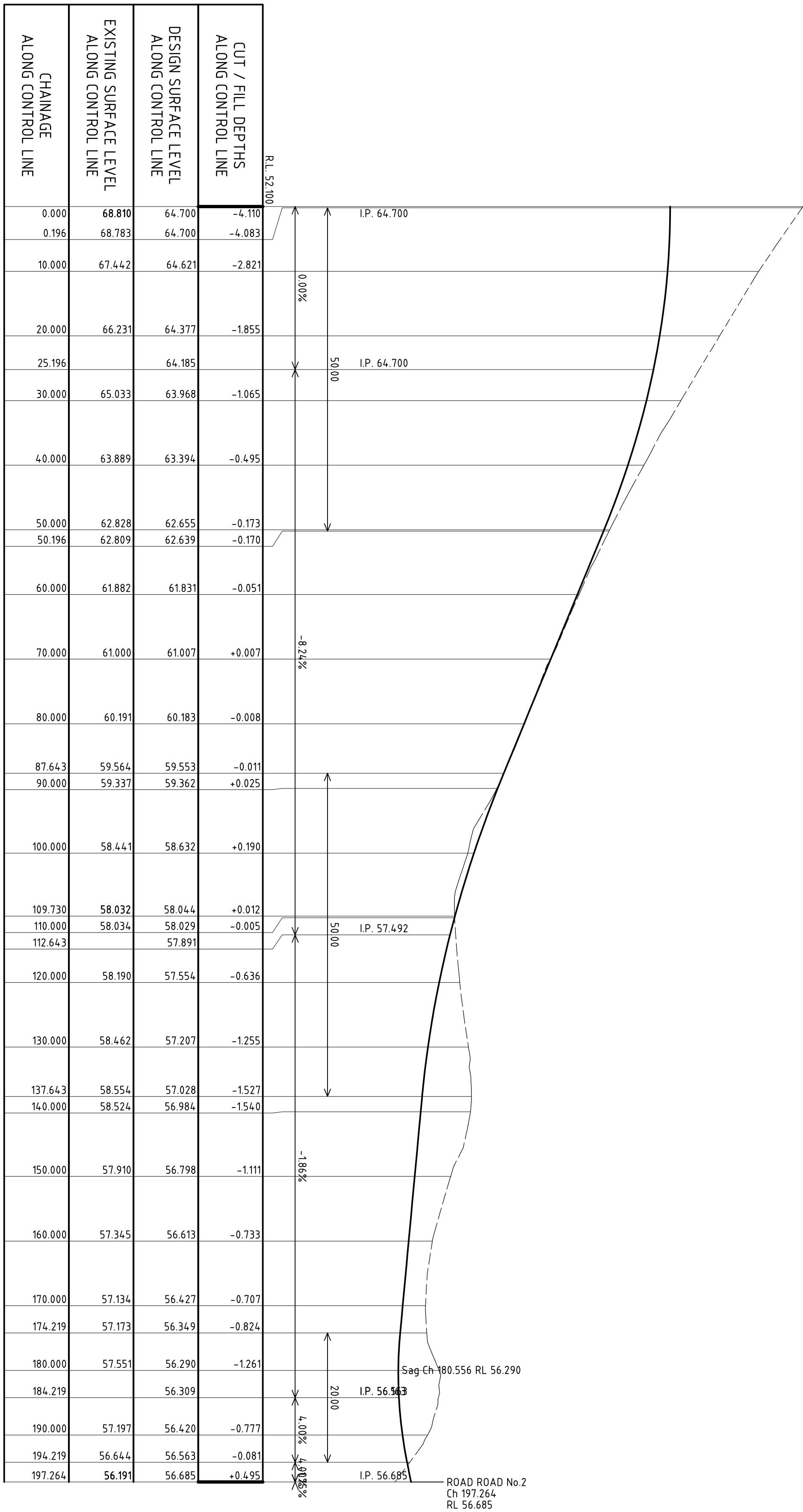
LONGITUDINAL SECTION ALONG ROAD No.3
