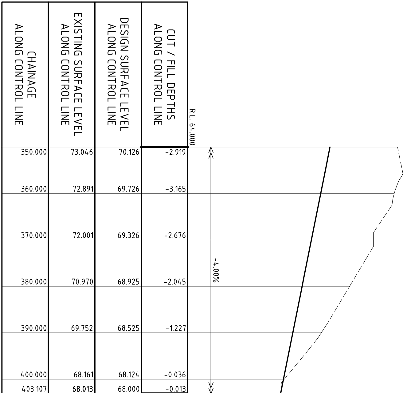
LONGITUDINAL SECTION ALONG ROAD No.5
