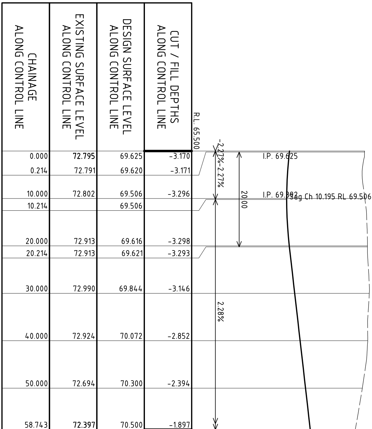
LONGITUDINAL SECTION ALONG ROAD No.6
