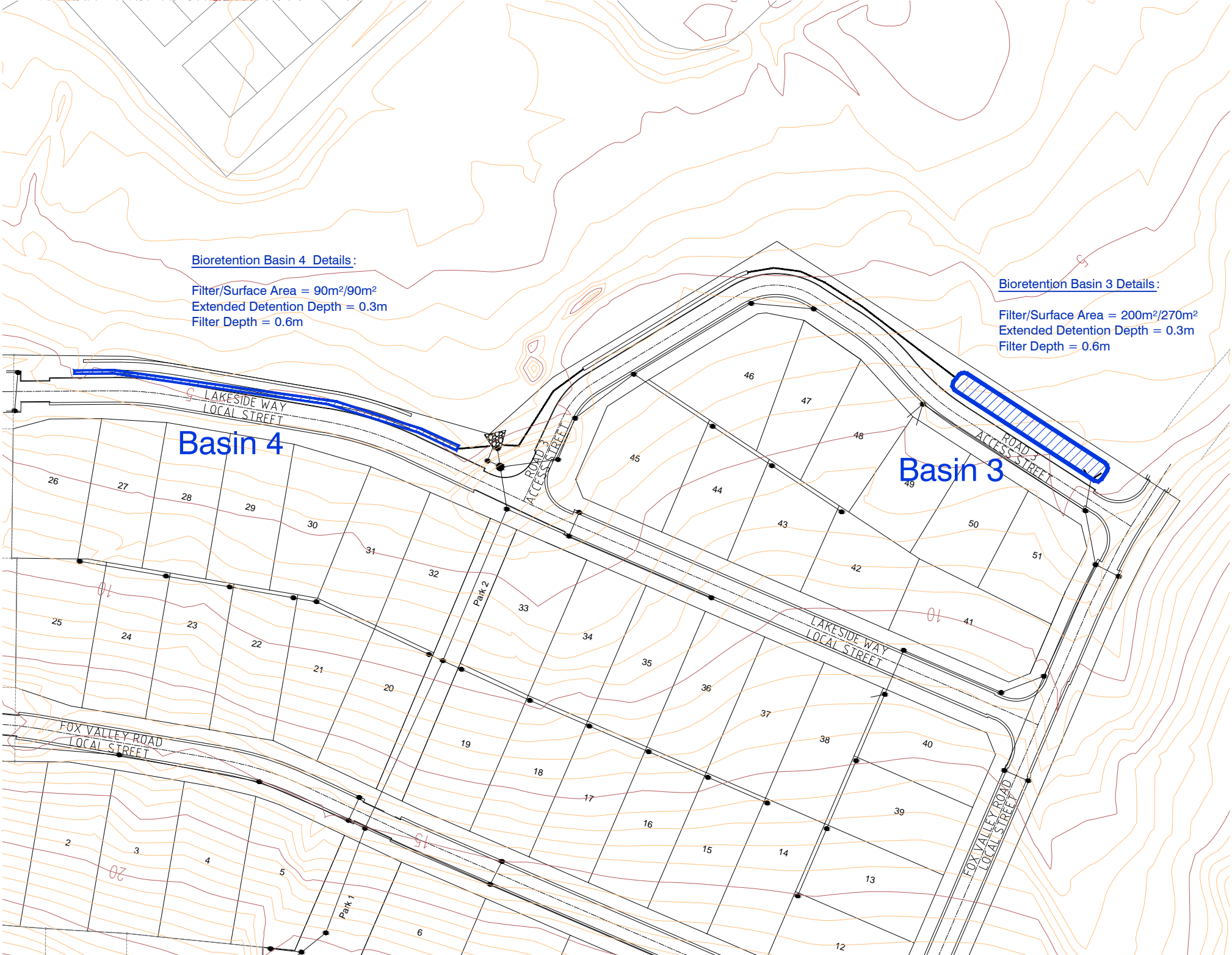
TYPICAL BIORETENTION BASIN FILTER ZONE DETAIL
