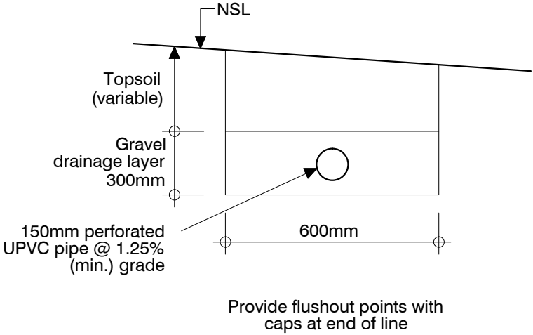
INFILTRATION TRENCH TYPICAL DETAIL
