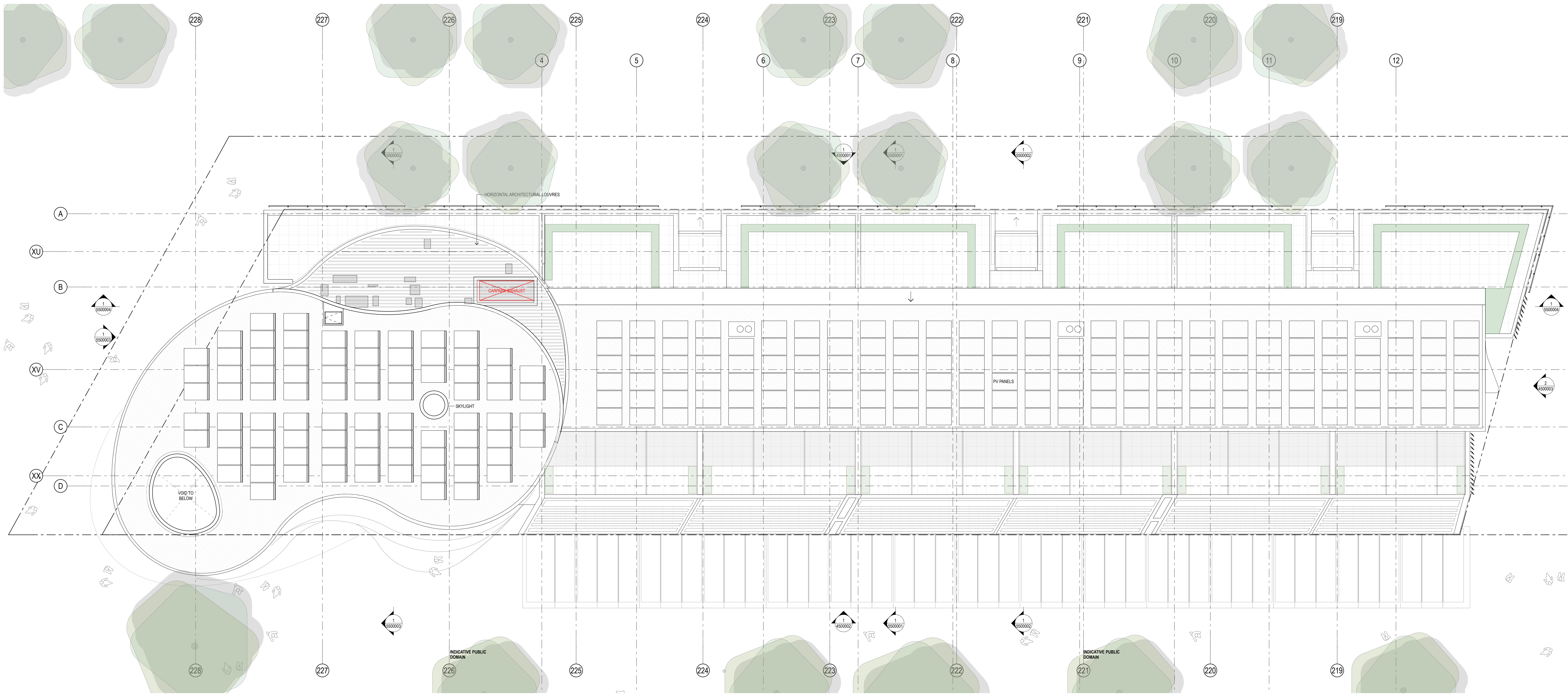
1 PLAN Roof 1:100
