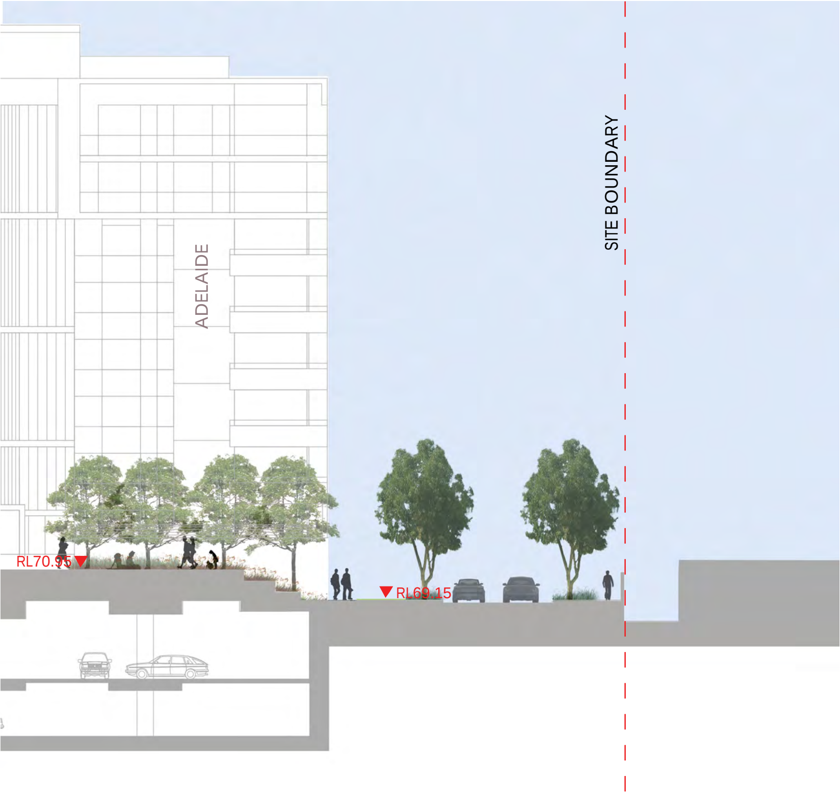
SECTION C
