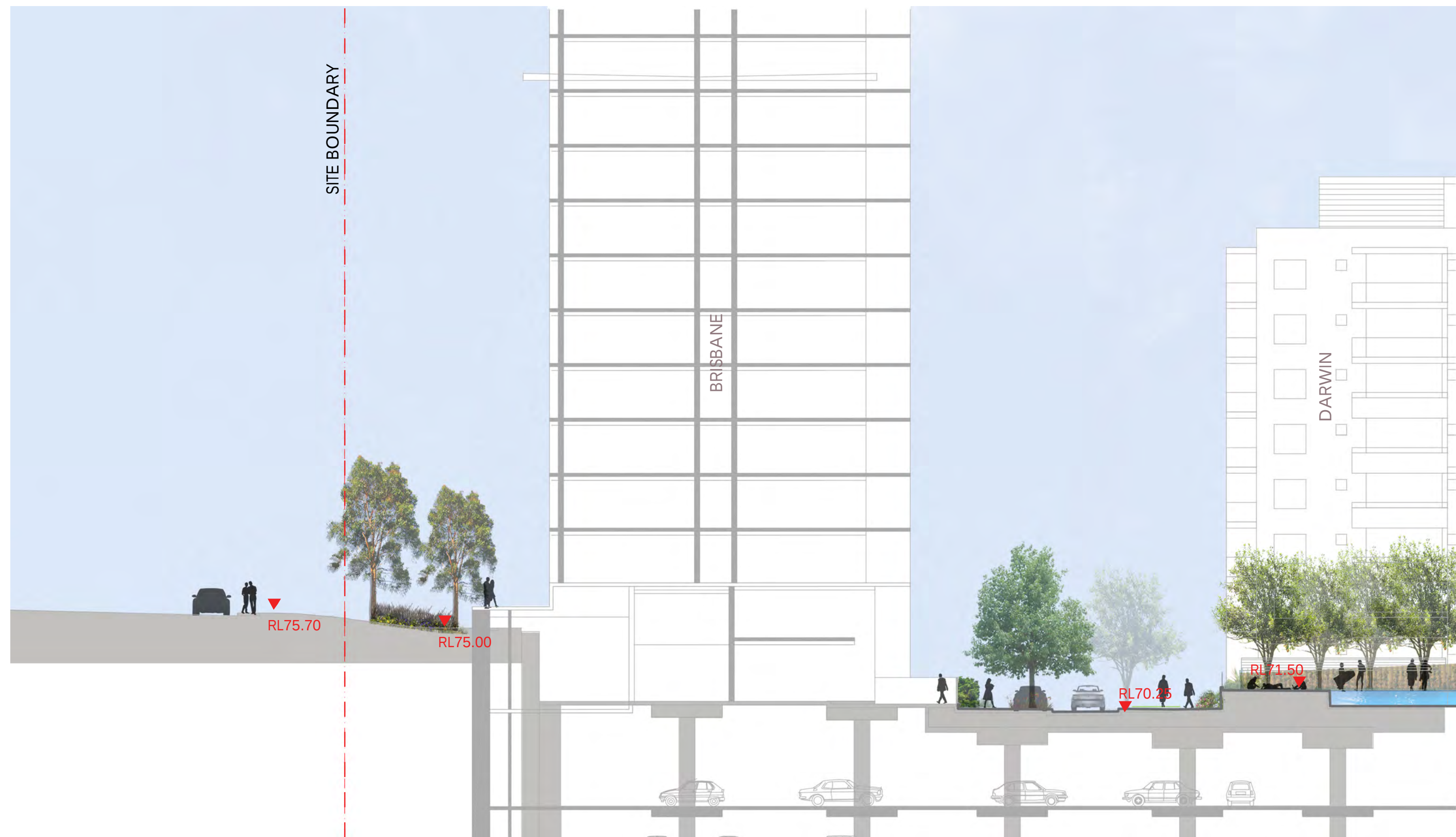
SECTION H
