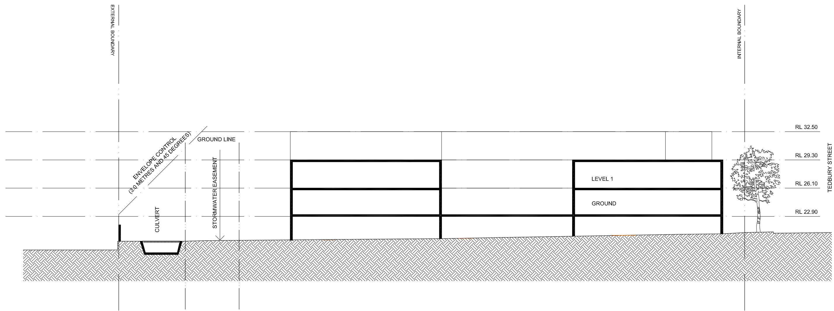
SECTION HH LOT 31 SENIORS LIVING COMPLEX
