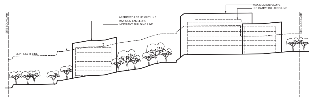
Section CC
