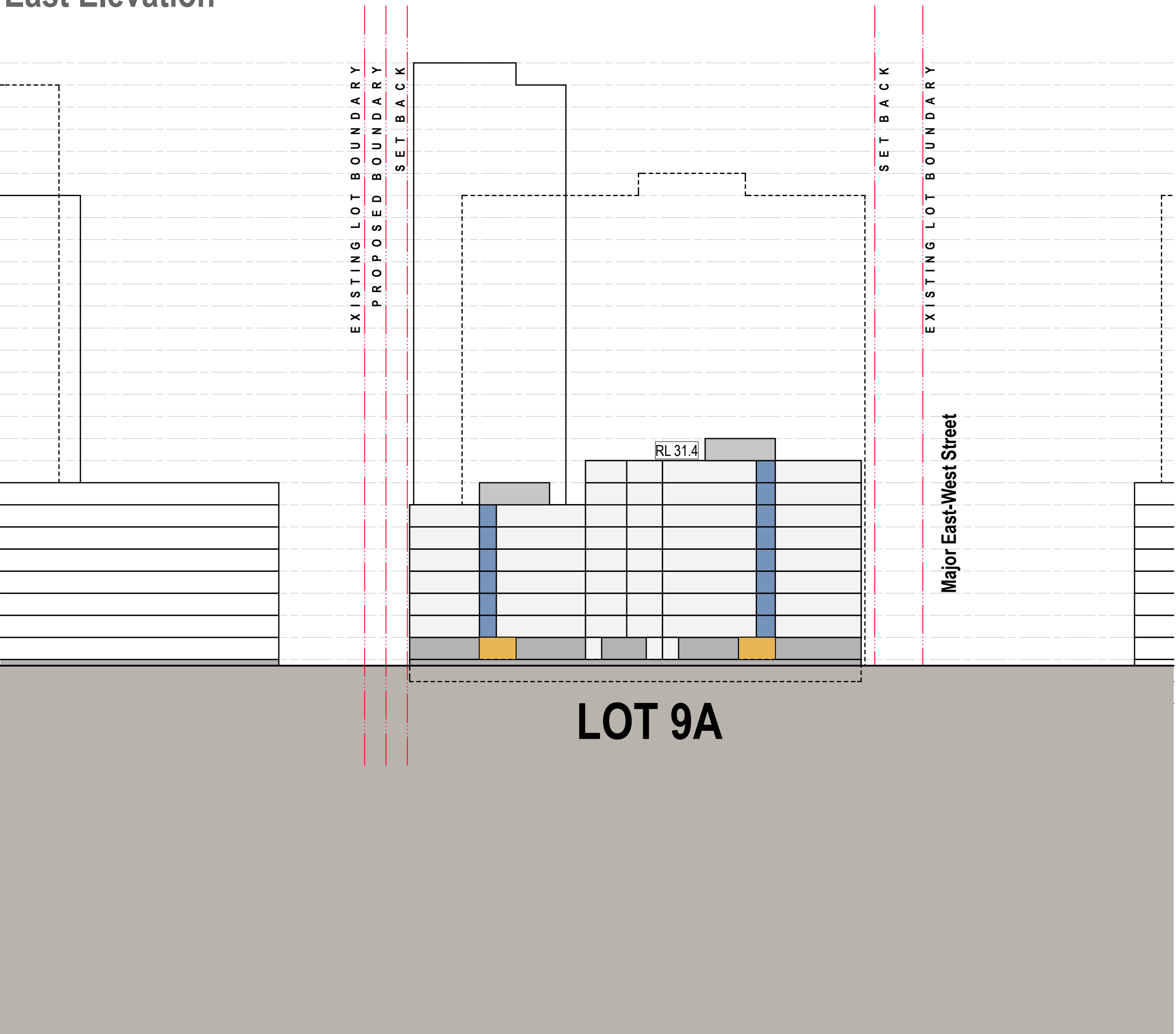
West Elevation
