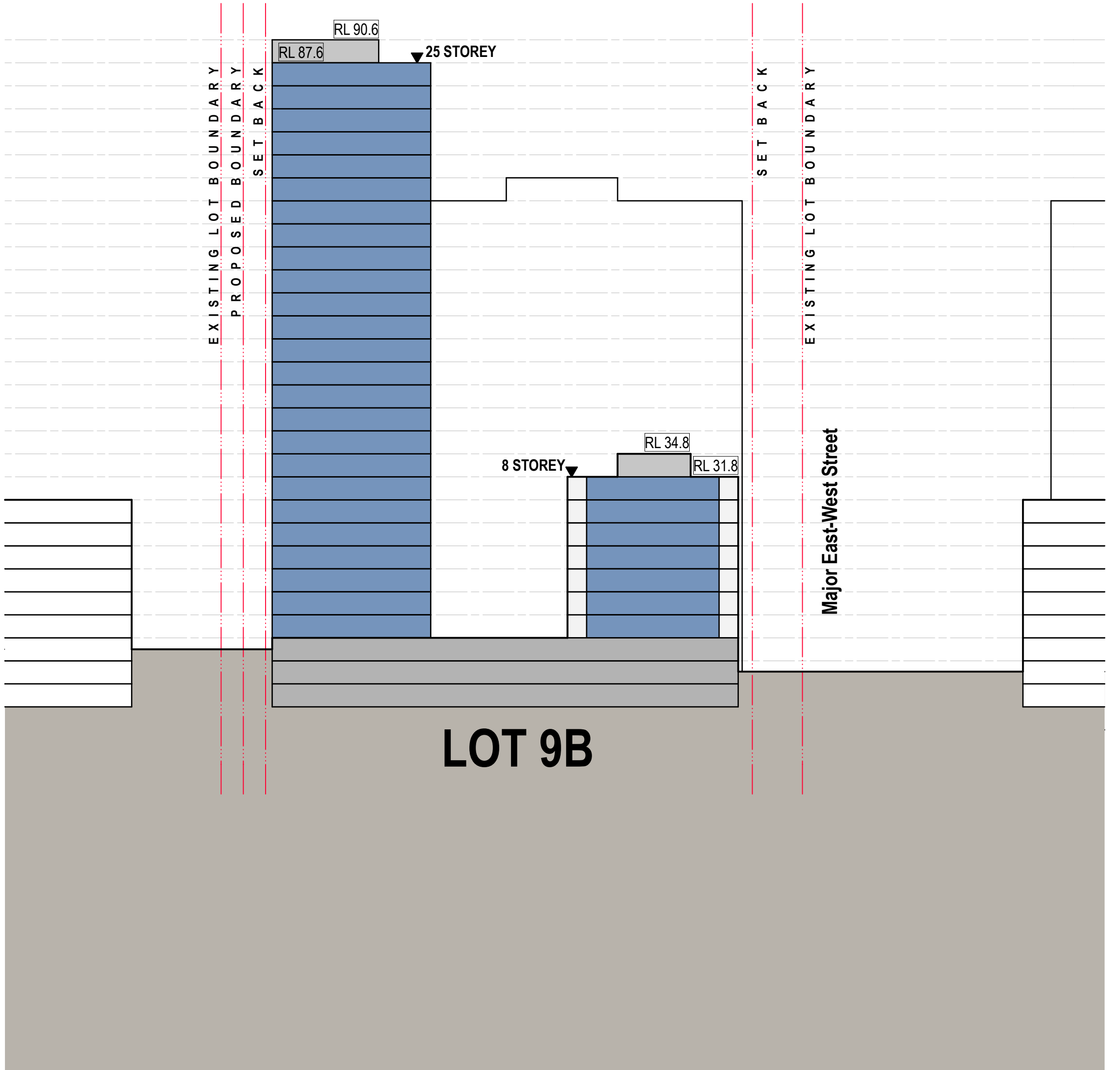
Section B
