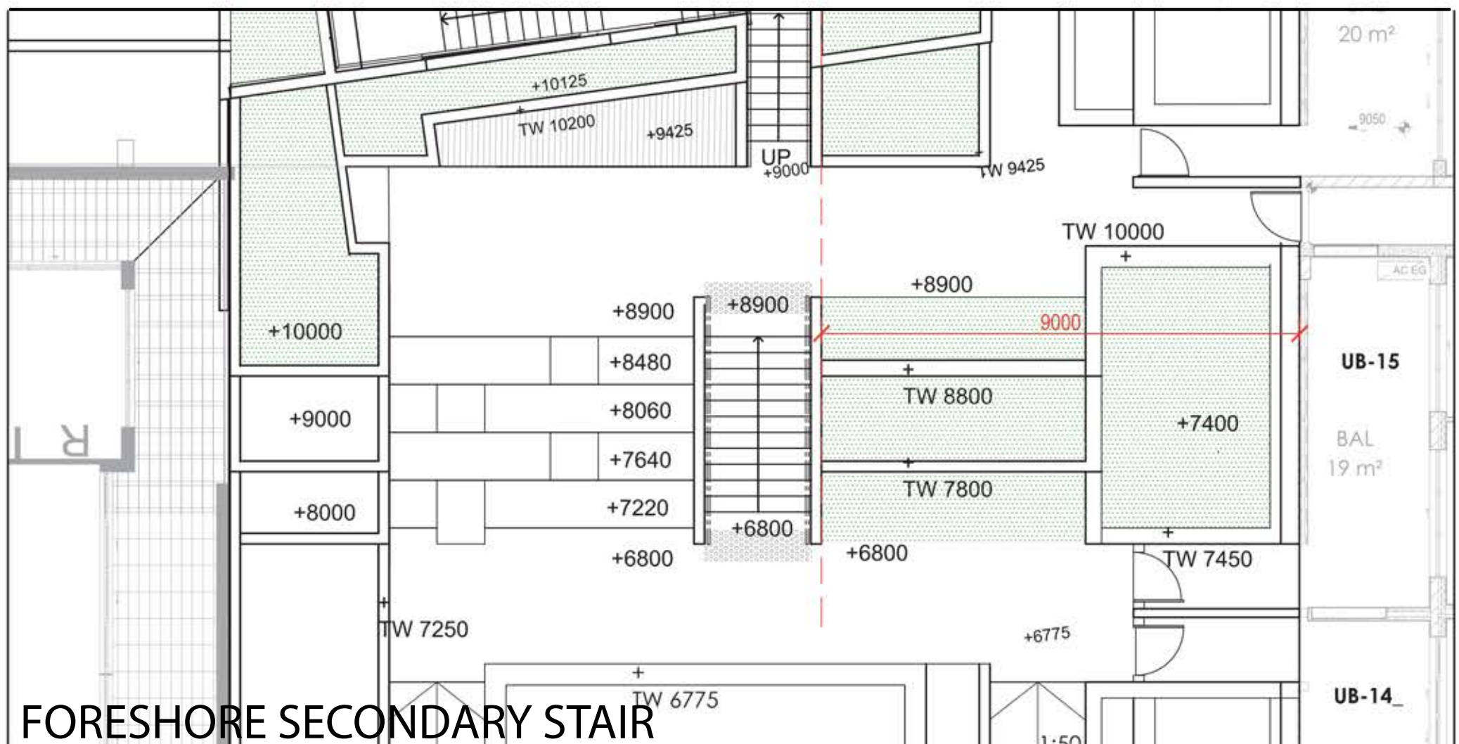
NEW FORESHORE LINK STAIRS
