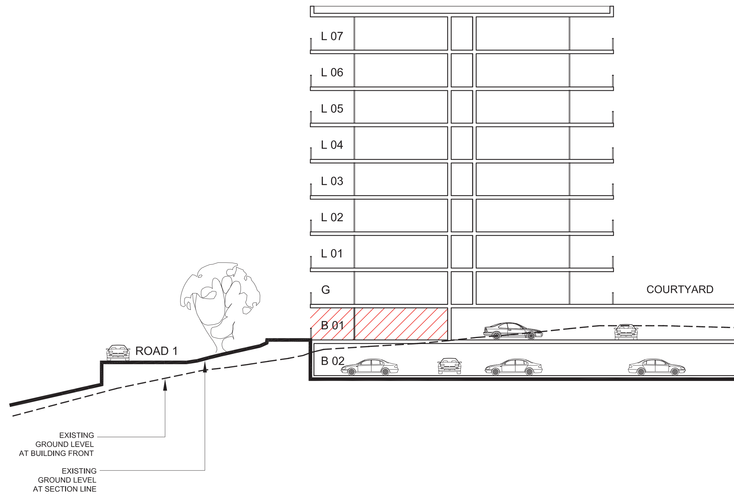
Section BB
