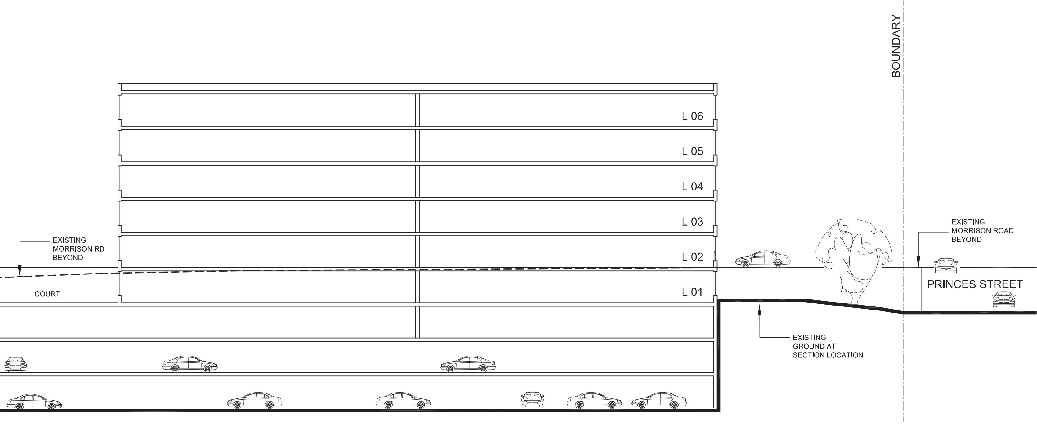
Section EE
