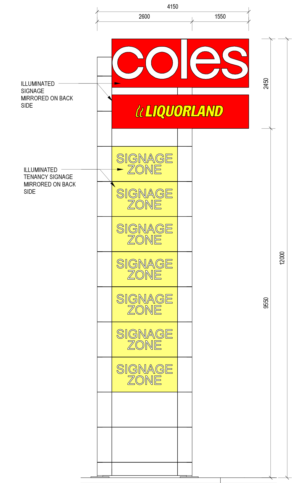
2 PYLON SIGN- FRONT ELEVATION 1 : 50
