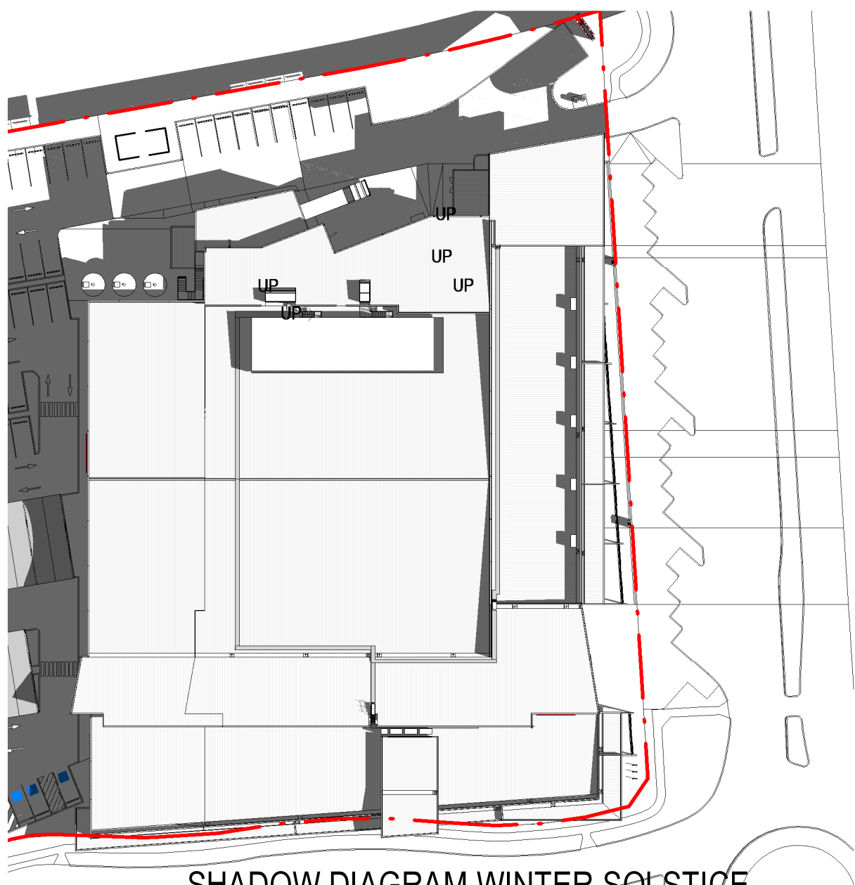
7 SHADOW DIAGRAM WINTER SOLSTICE 10.00am 1 : 750
