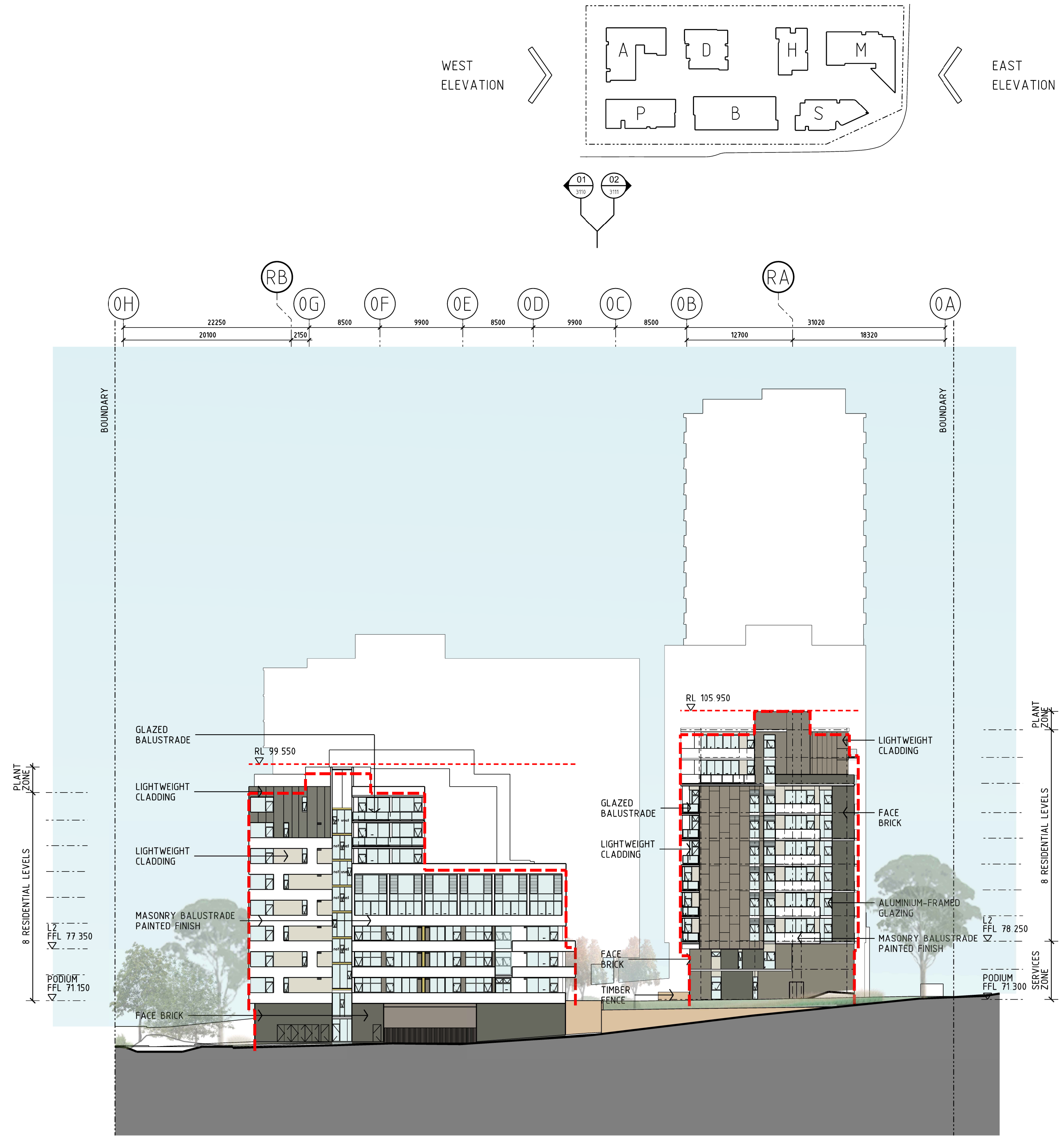
BUILDING ADELAIDE BUILDINGS DARWIN, HOBART AND MELBOURNE BEYOND BUILDING PERTH BUILDINGS BRISBANE AND SYDNEY BEYOND WEST ELEVATION
