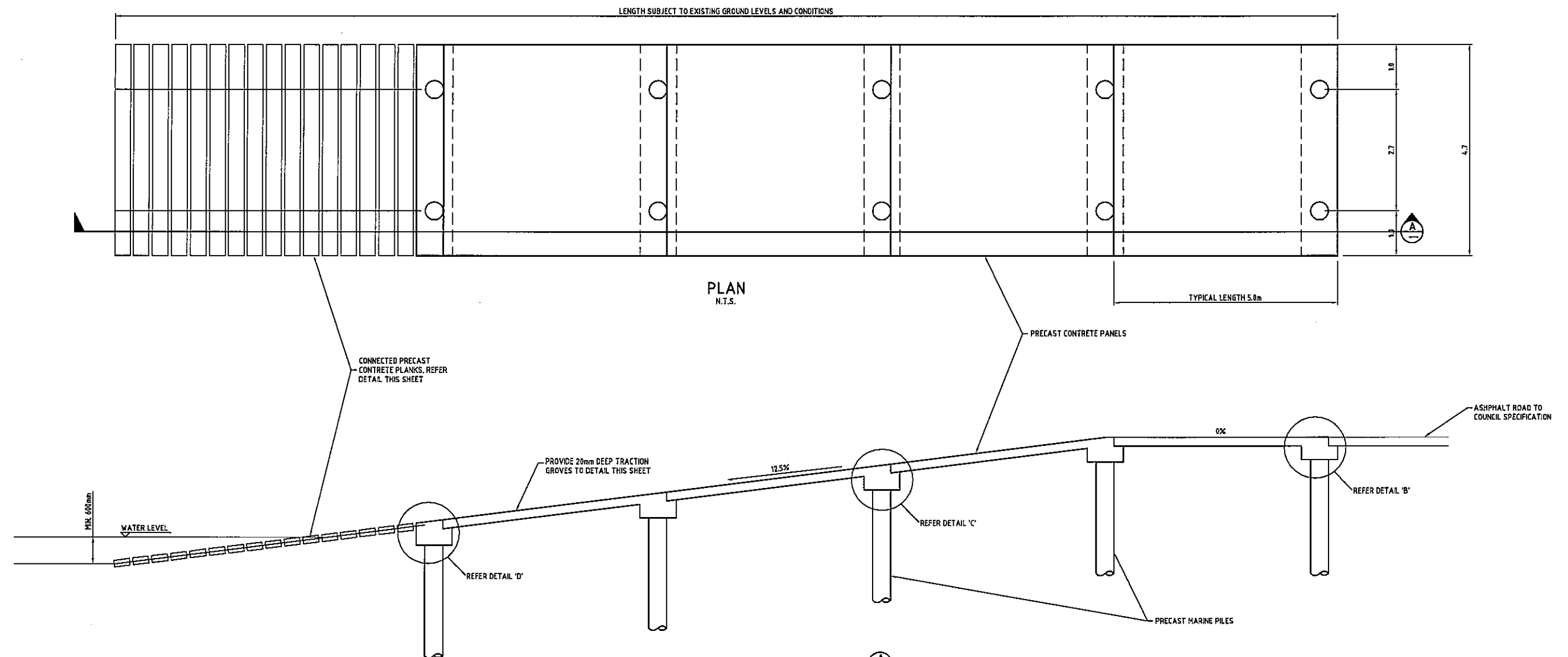
SECTION A BOAT RAMP ELEVATION N.T.S.
