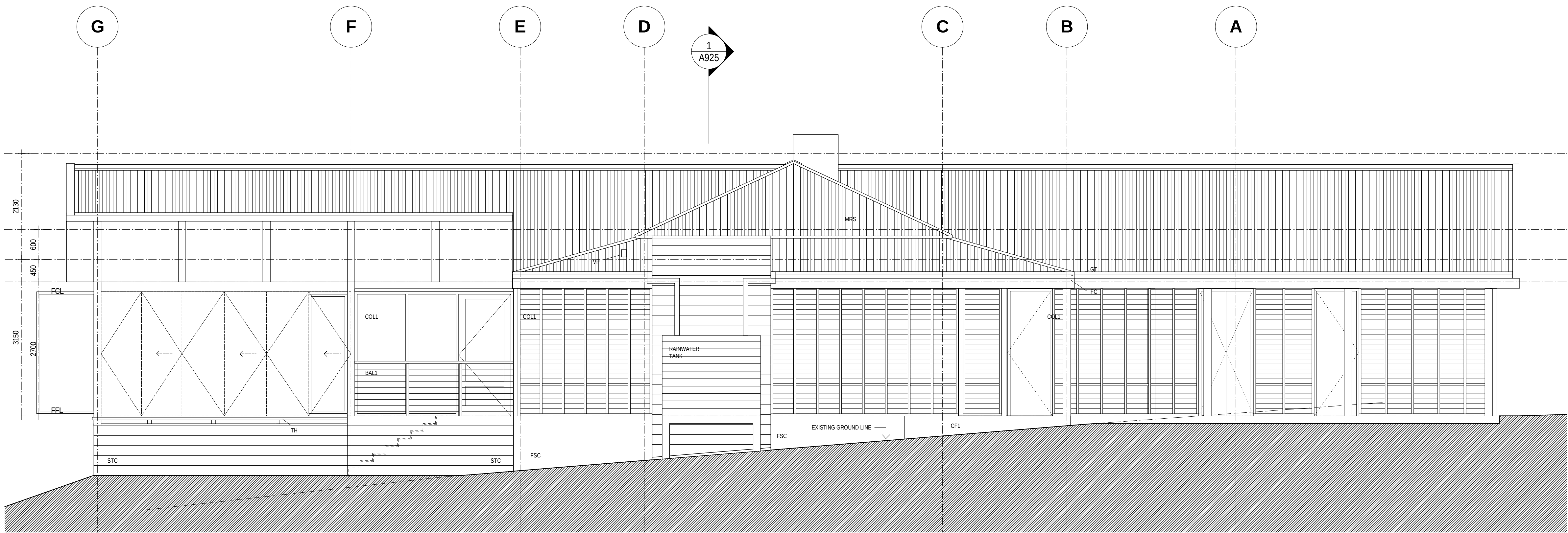
1 ELEVATION 2 SCALE 1:50
