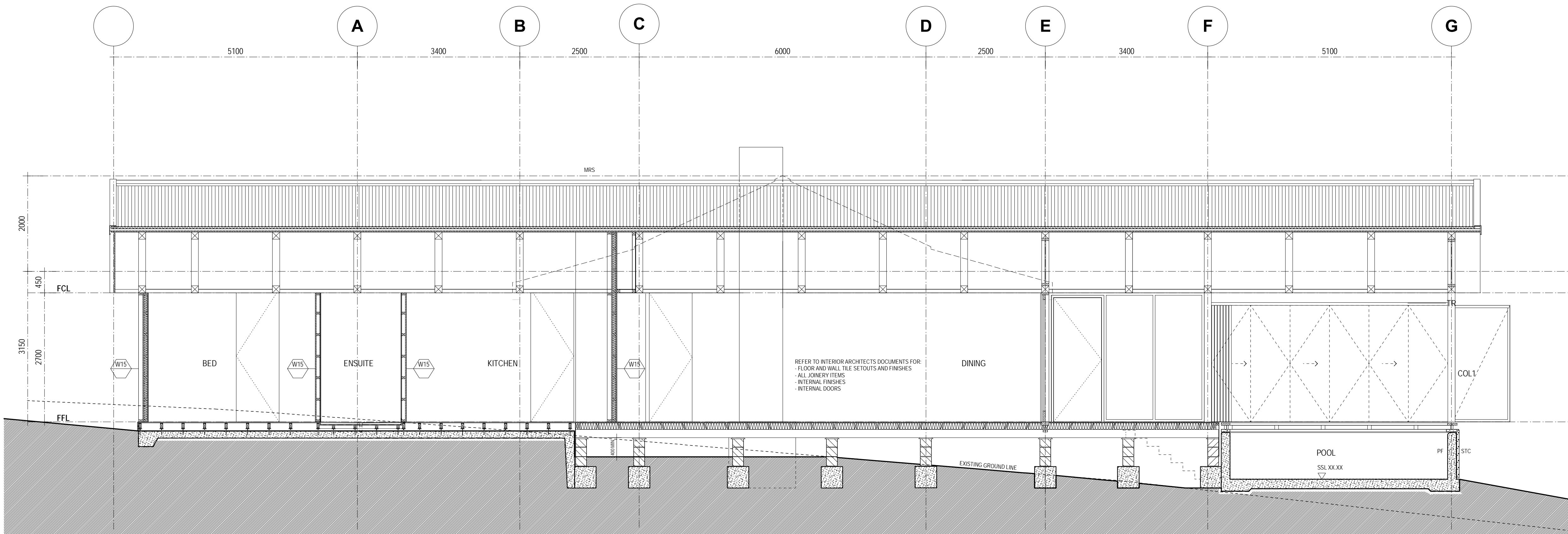
2 SECTION B-B SCALE 1:50
