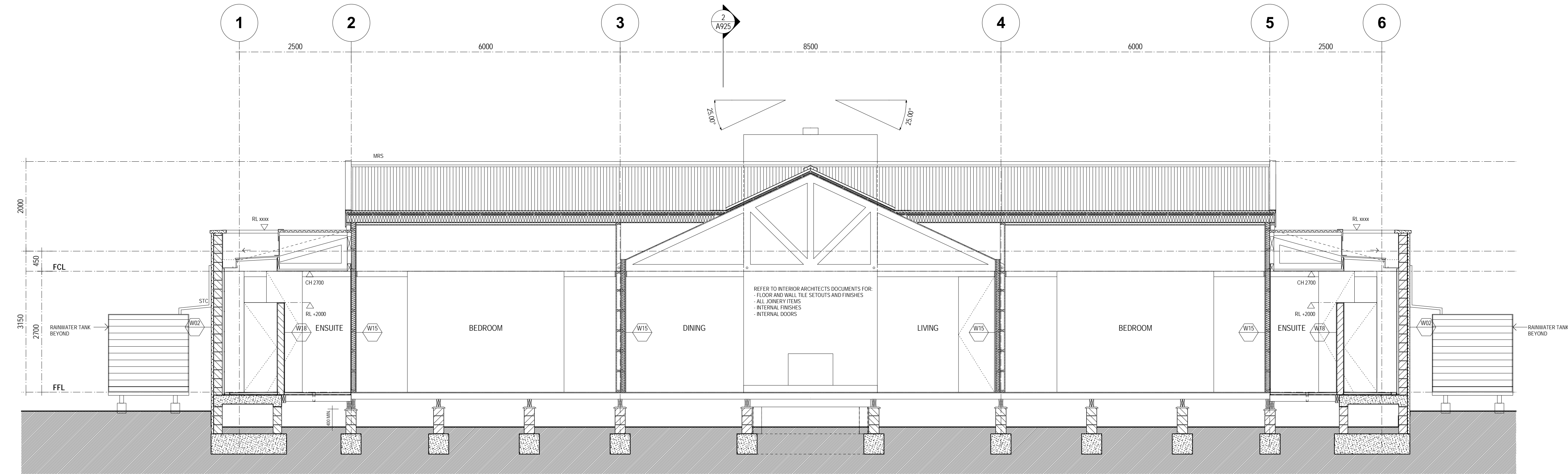
1 SECTION A-A SCALE 1:50
