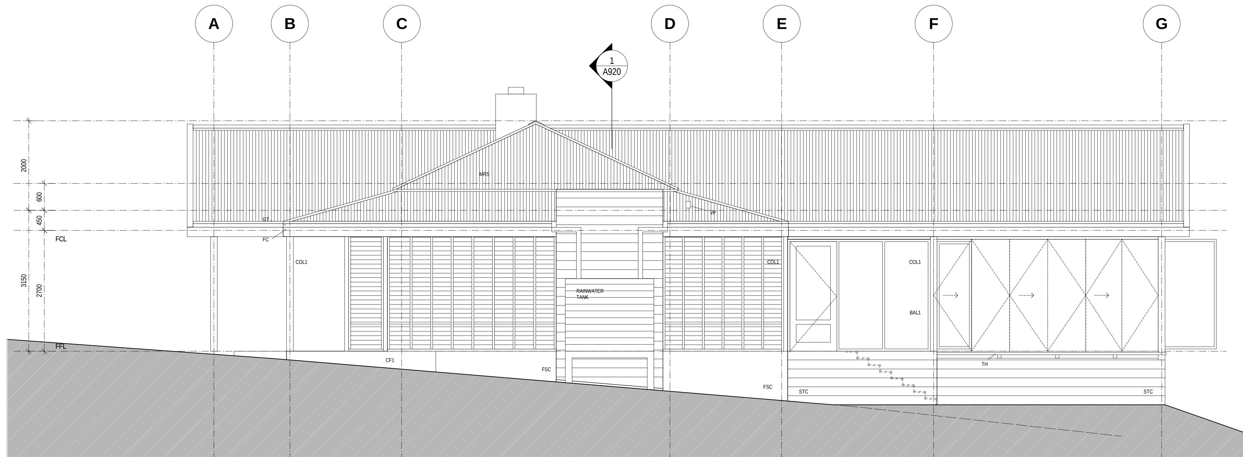
2 ELEVATION 4 SCALE 1:50
