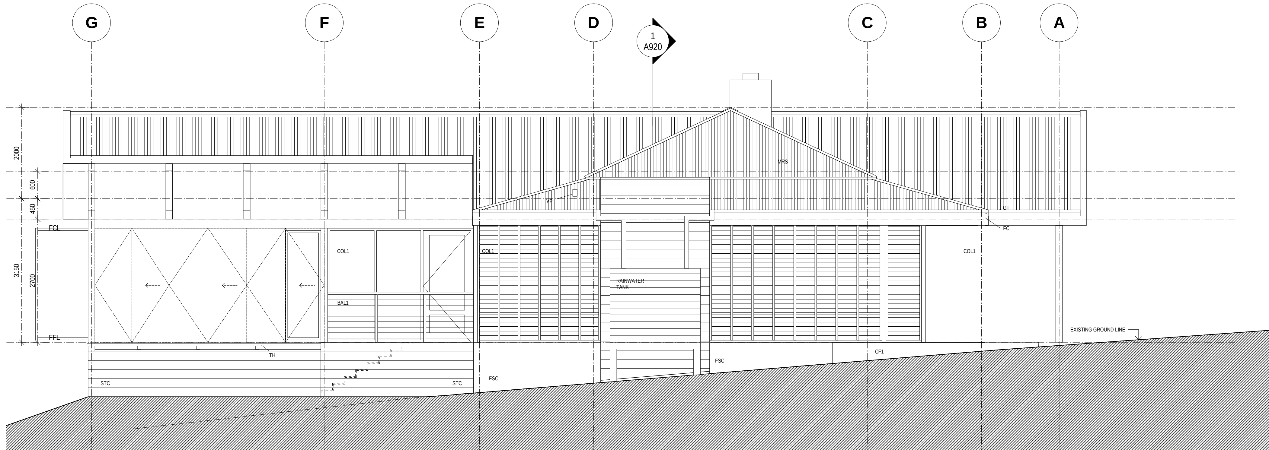
1 ELEVATION 2 SCALE 1:50
