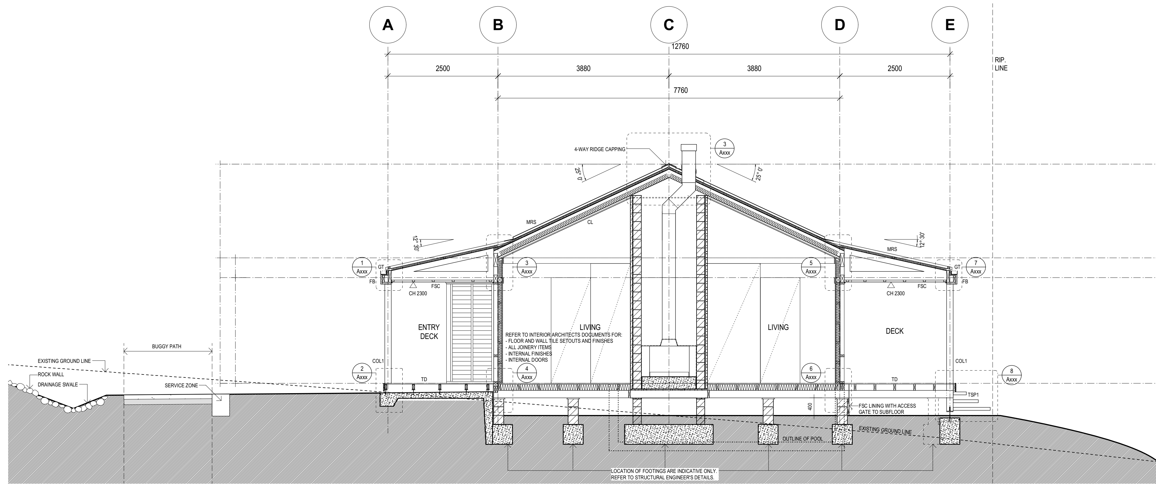
2 SECTION B-B SCALE 1:50
