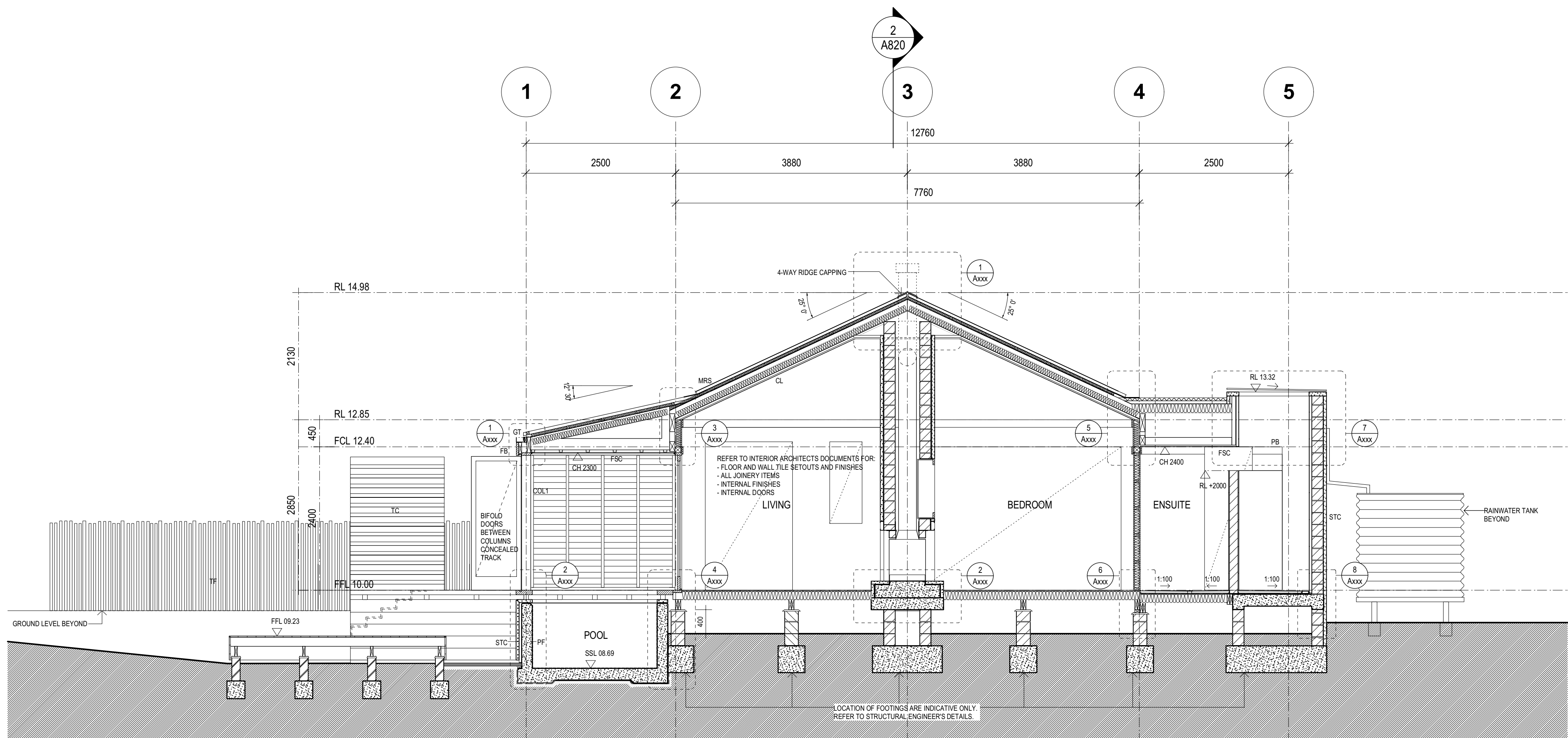
1 SECTION A-A SCALE 1:50
