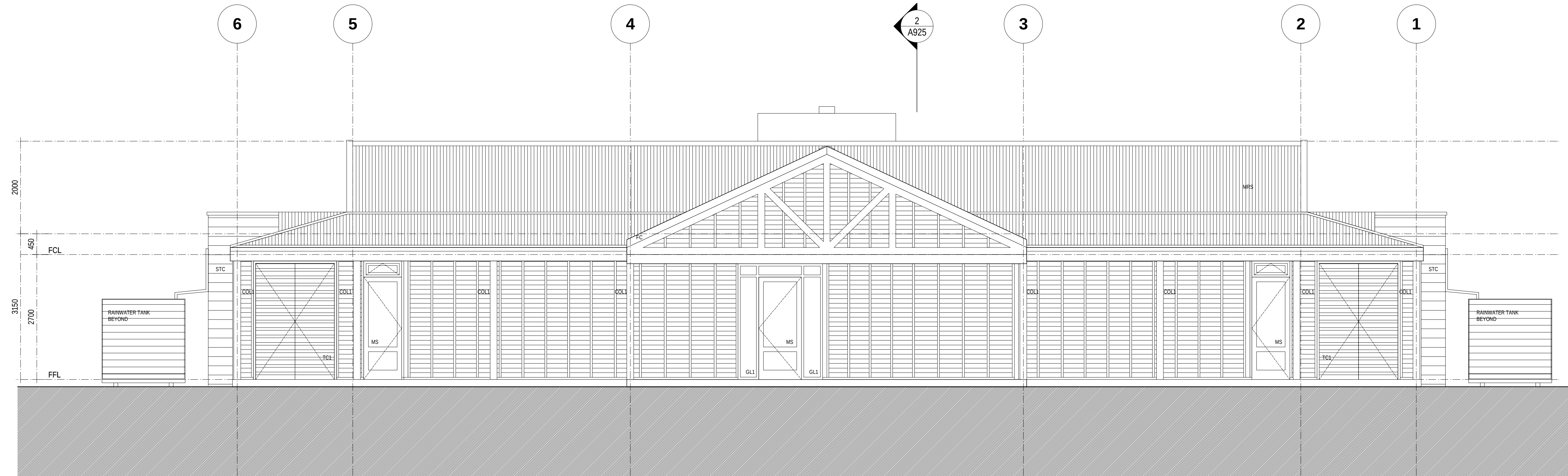
2 ELEVATION 3 - SCALE 1:50
