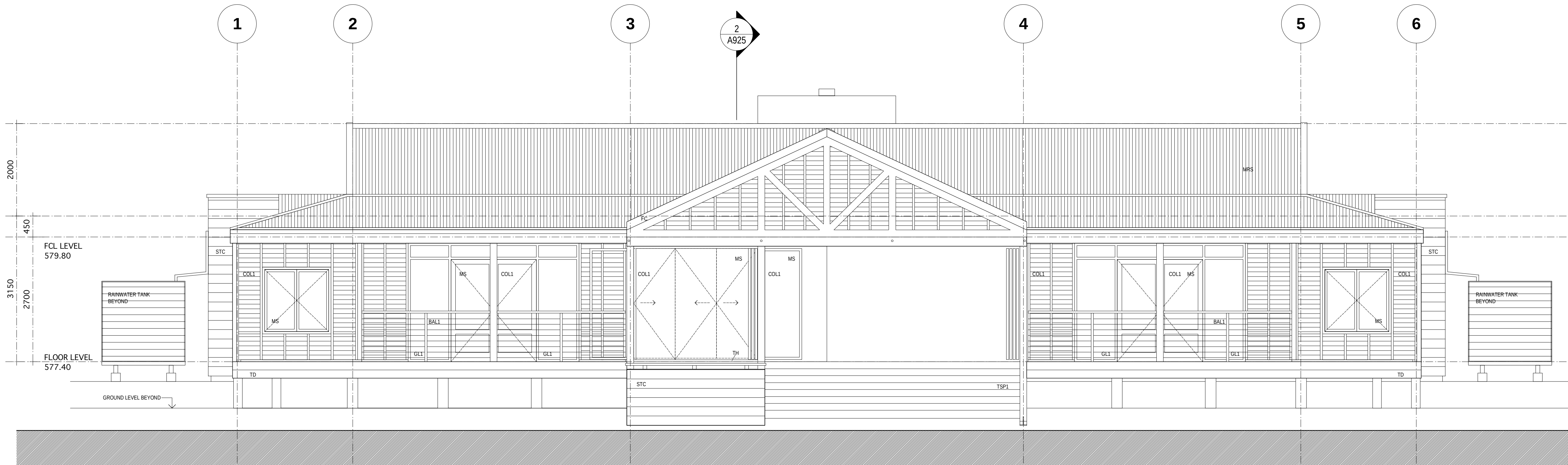
1 ELEVATION 1 - SCALE 1:50
