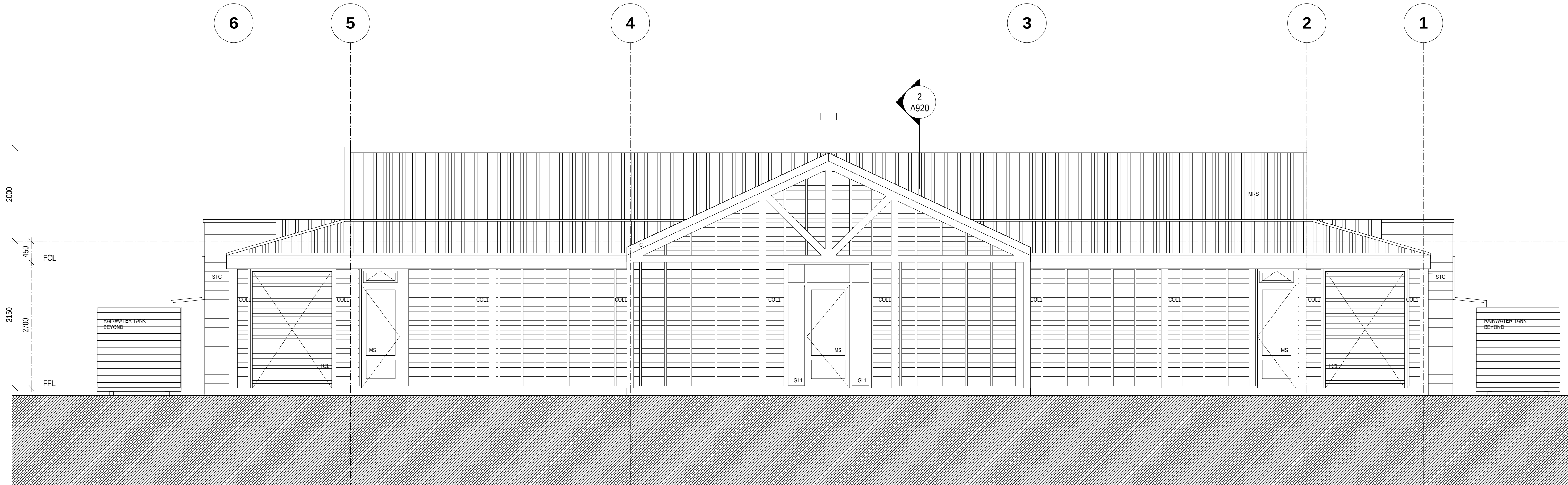
2 ELEVATION 3 - SCALE 1:50
