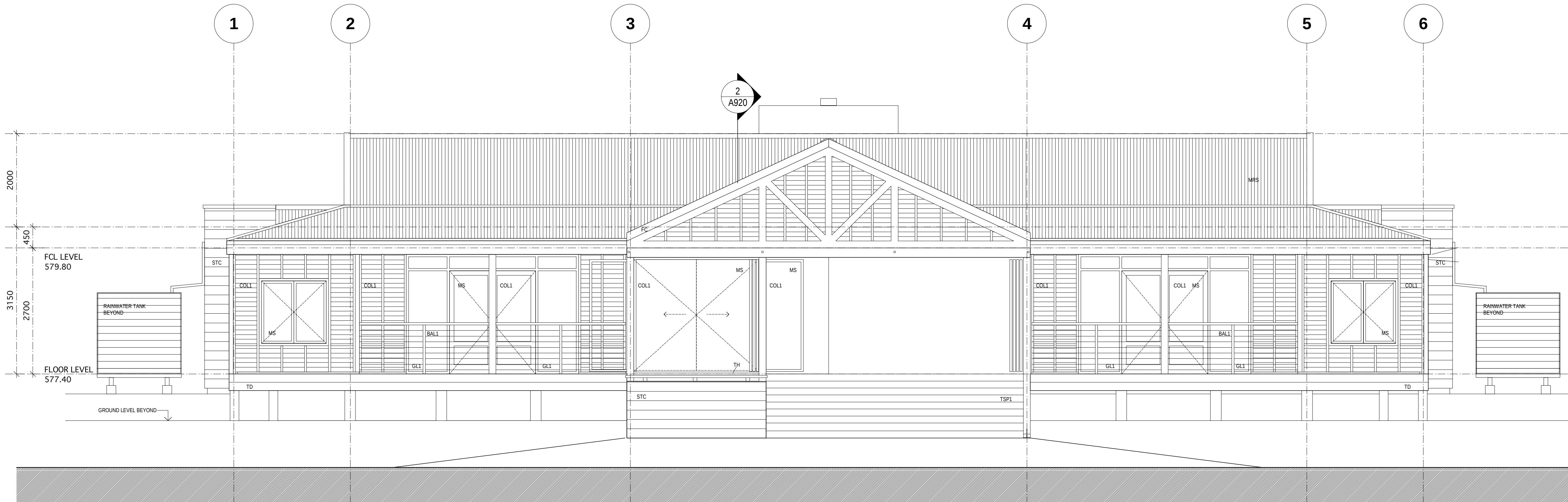
1 ELEVATION 1 - SCALE 1:50
