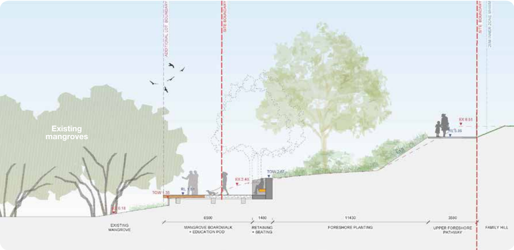
Mangrove Boardwalk | Section GG
