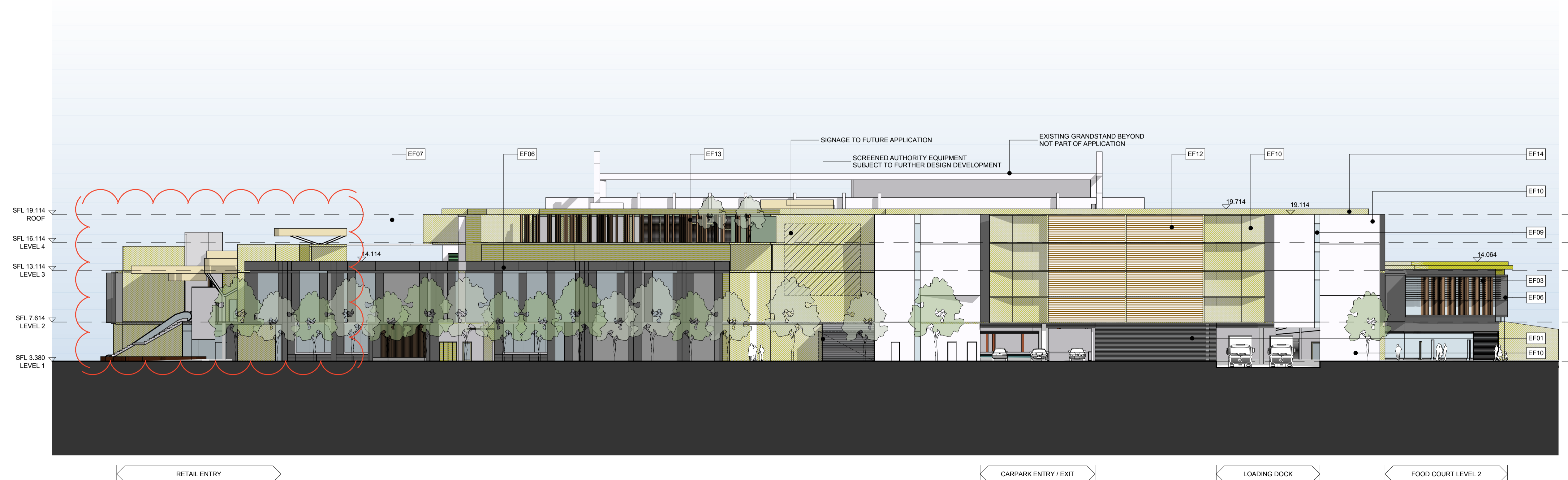
2 ELEVATION WOOLLOOWARE ROAD NORTH ELEVATION (EAST) 1:250
