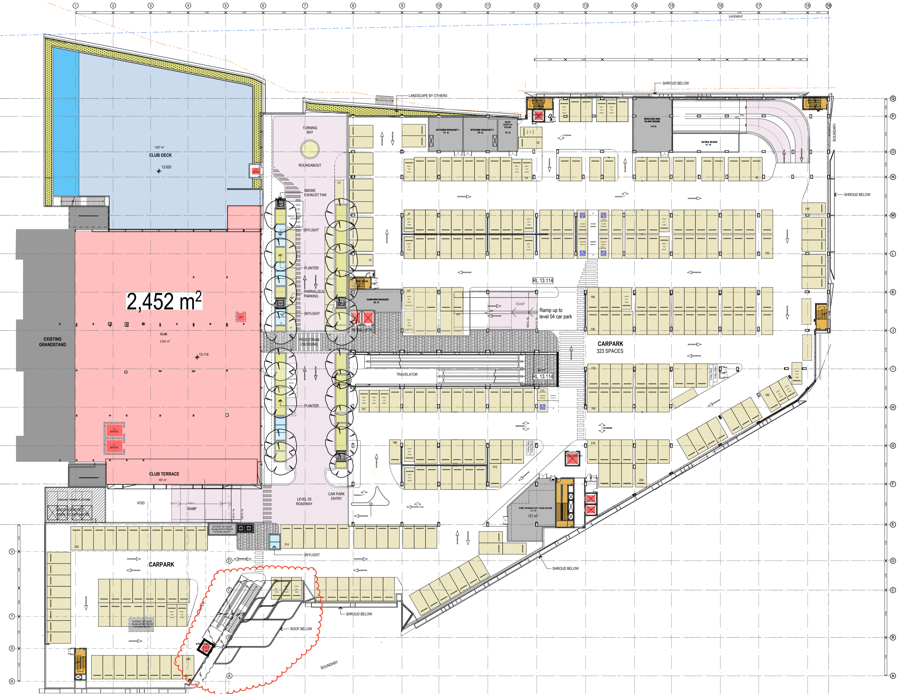
3 PLAN GFA LEVEL 3 1:500
