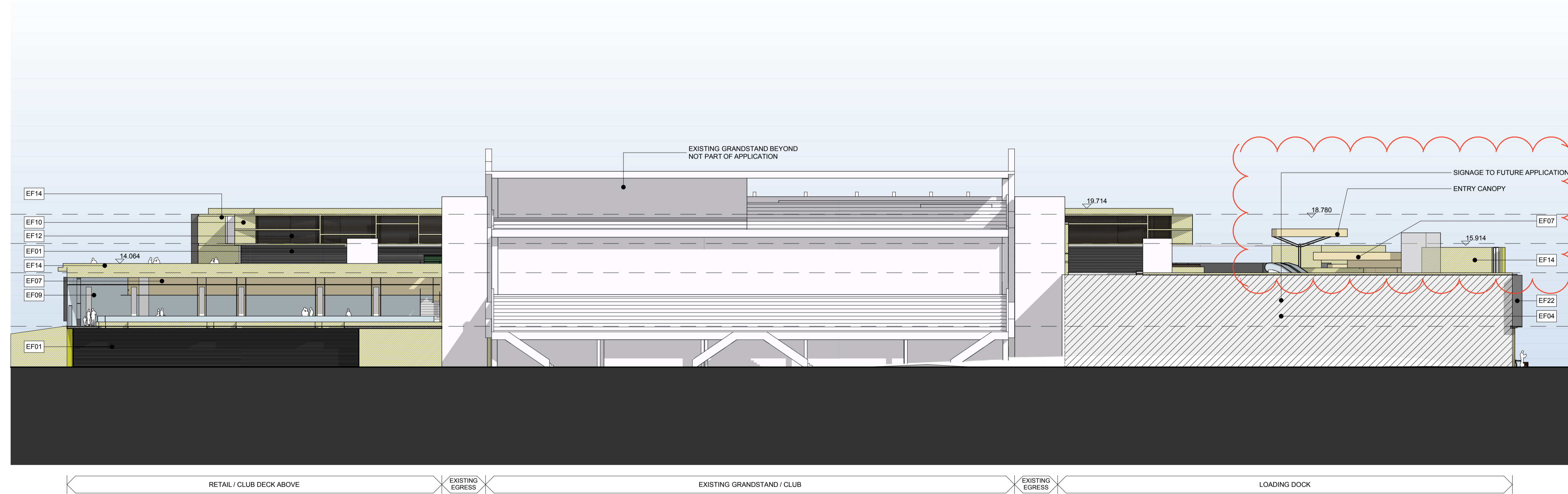
2 ELEVATION SHARKS STADIUM ELEVATION (WEST) 1:250
