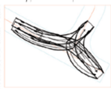
INSERT A- SERVICE VEHICLE TURNING PATH SCALE 1:500
