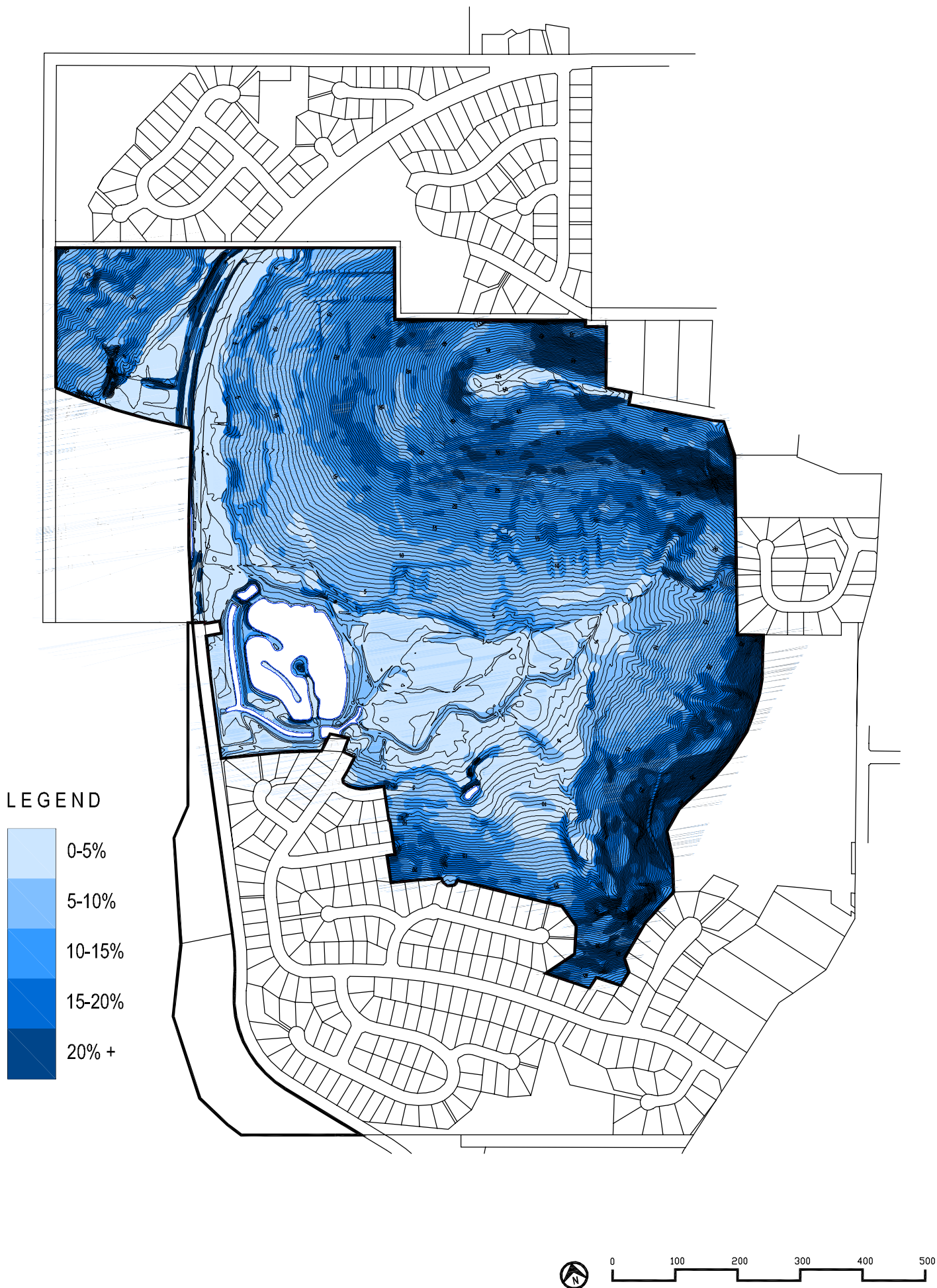
ILLUSTRATION 2.4 SLOPE ANALYSIS
