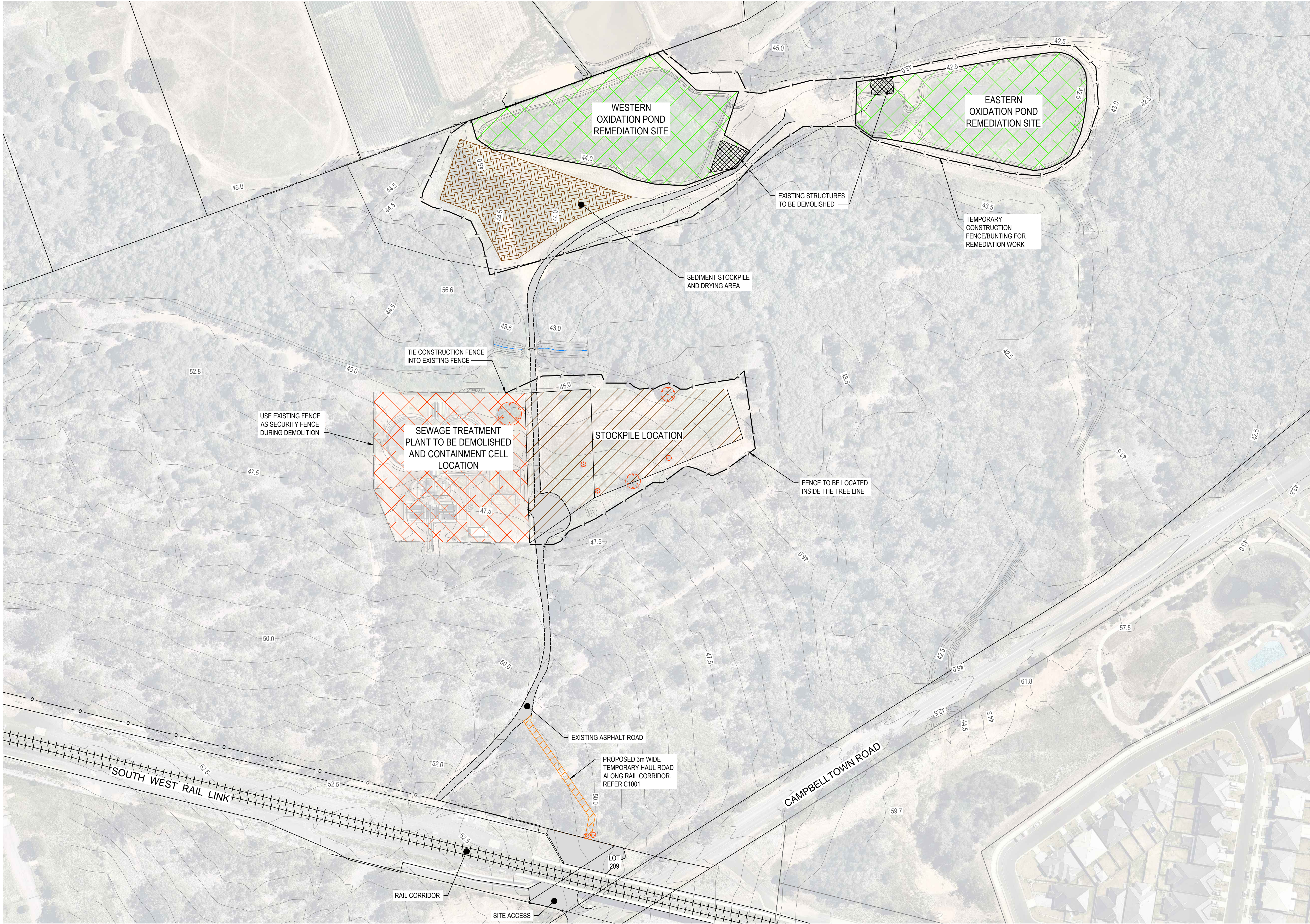
STP DEMOLITION AND OXIDATION POND REMEDIATION PLAN SCALE 1:1000
