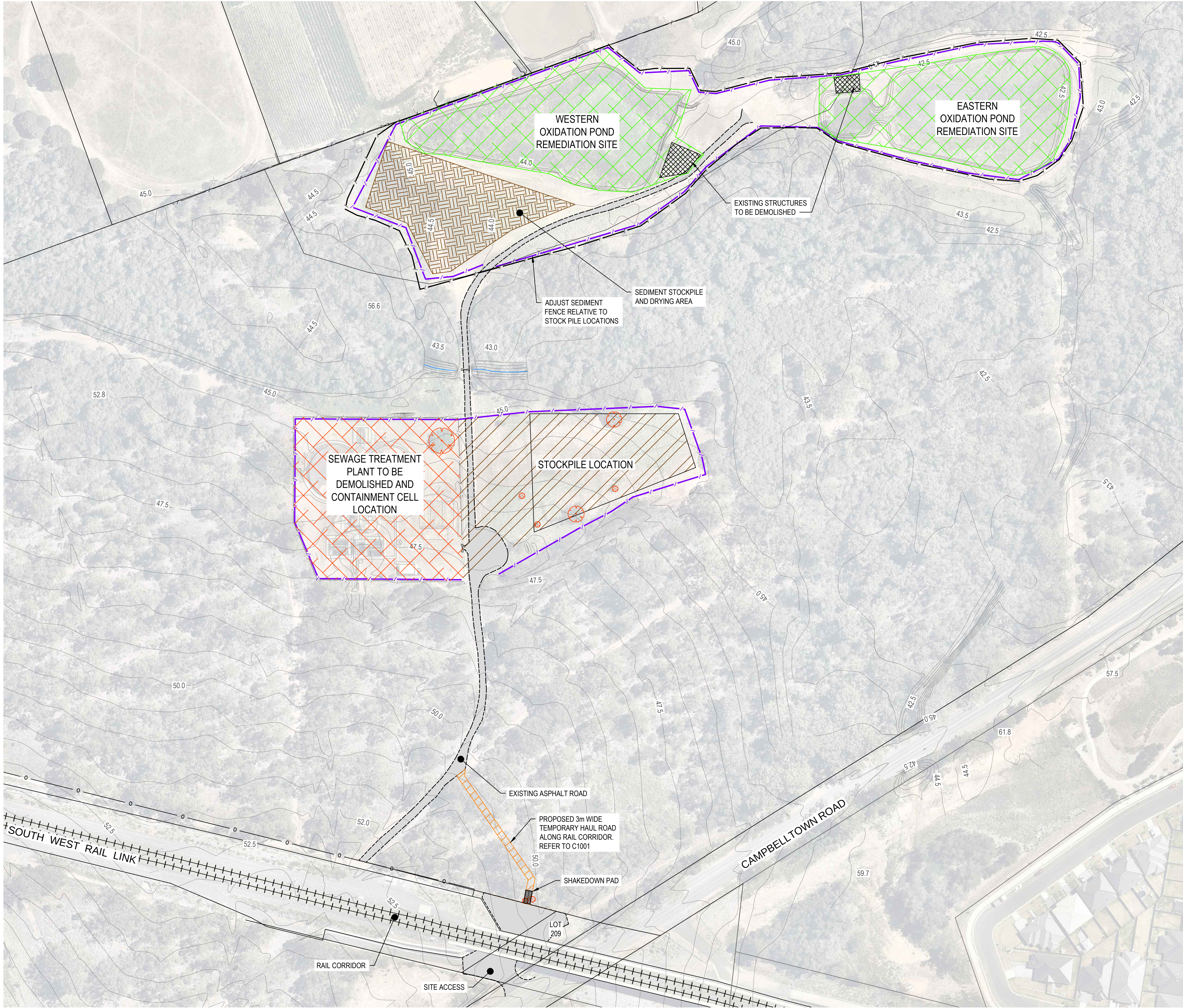
SOIL AND WATER MANAGEMENT PLAN SCALE 1:1000
