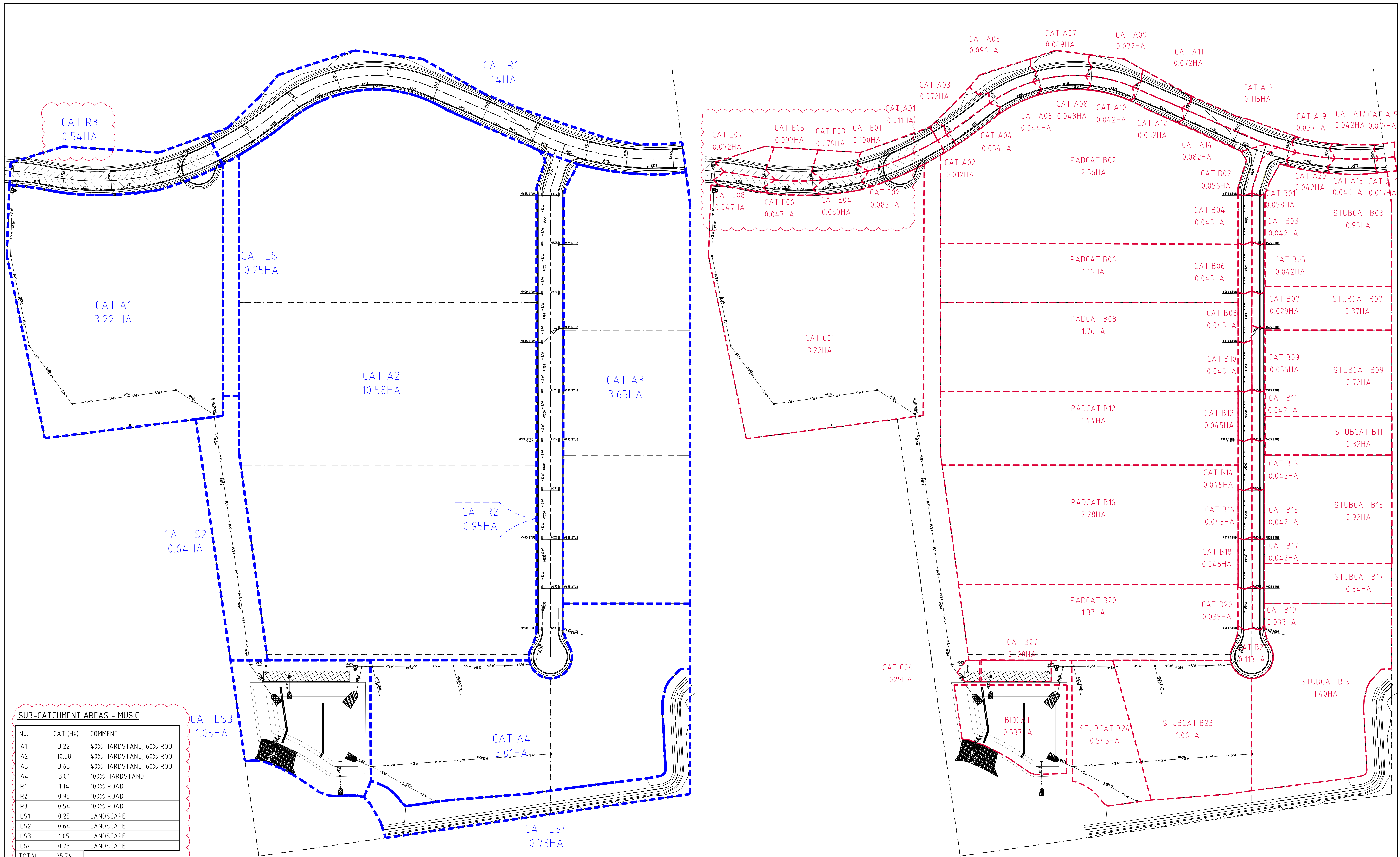
STORMWATER 'MUSIC' CATCHMENT PLAN SCALE 1:1000
