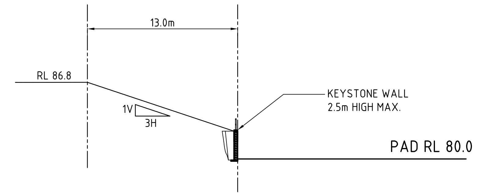
SECTION 1:200 1
