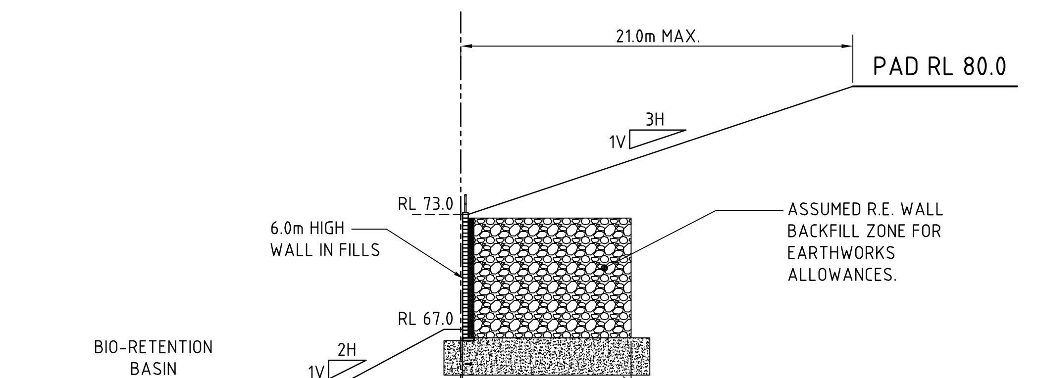
SECTION 1:200 2
