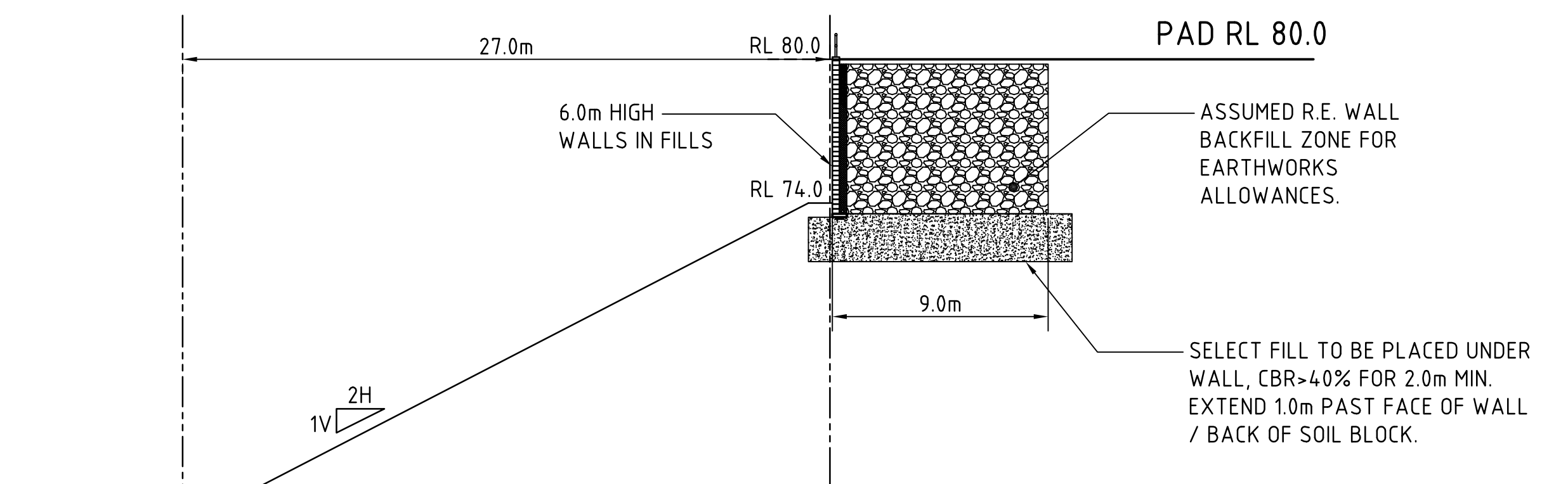
SECTION 1:200 2
