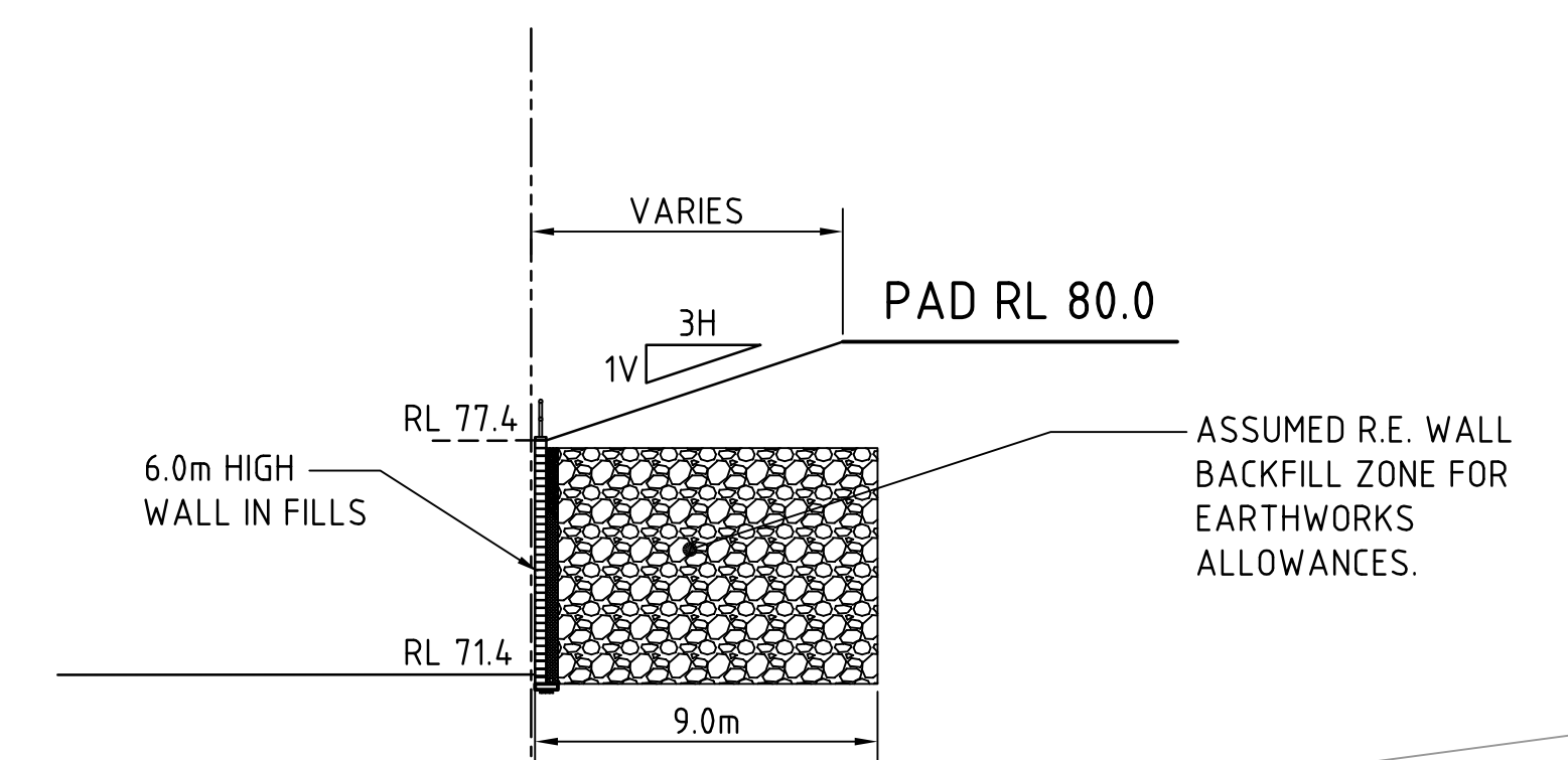
SECTION 1:200 3
