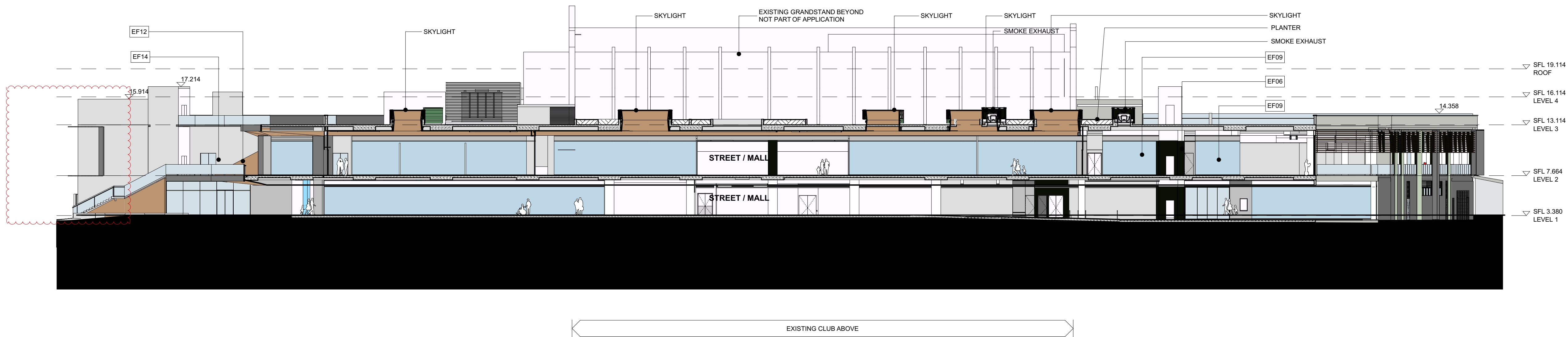
1 SECTION NORTH SOUTH 1:250
