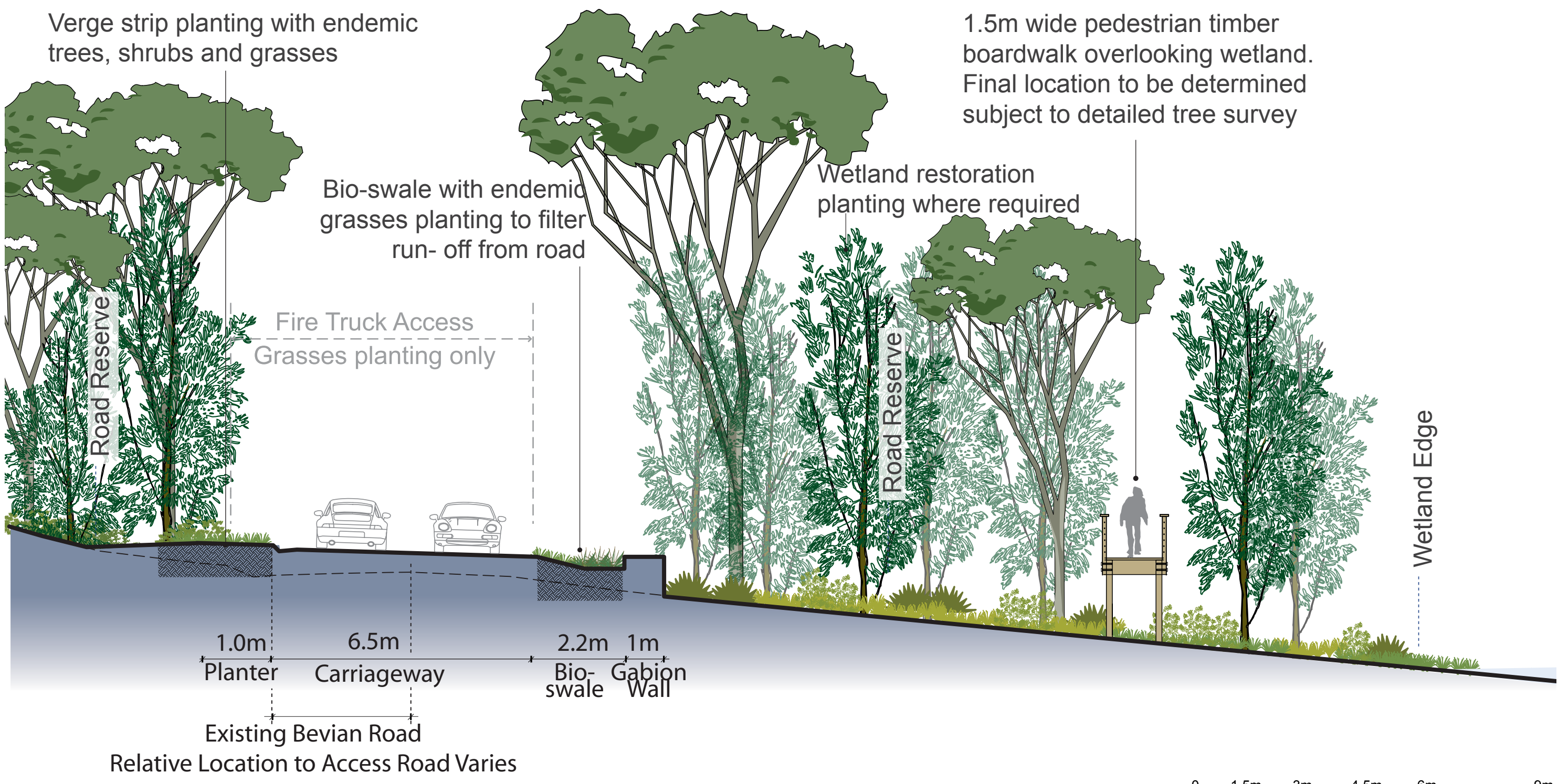
Section Through Southern Access Road - CH360
