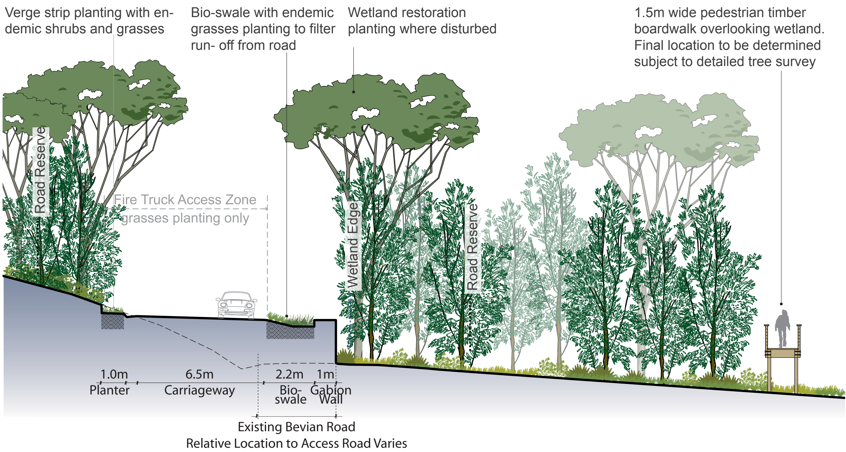
Section Through Southern Access Road - CH70
