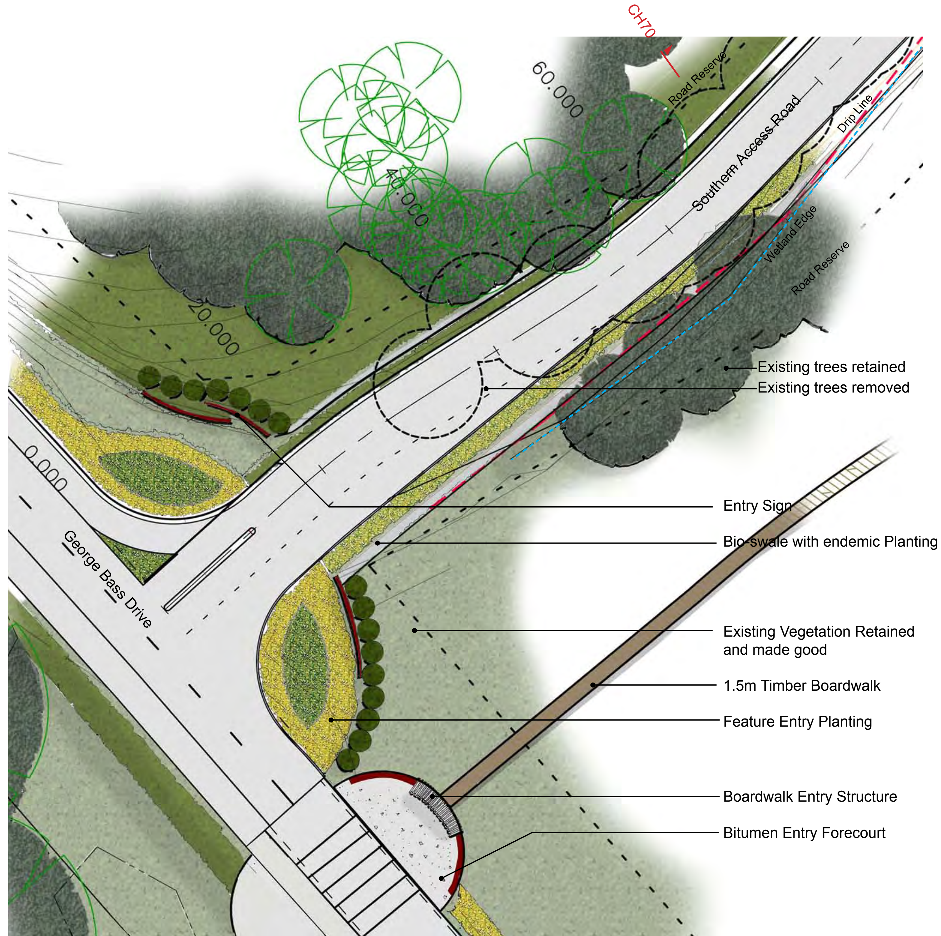
Southern Access Entry Detail
