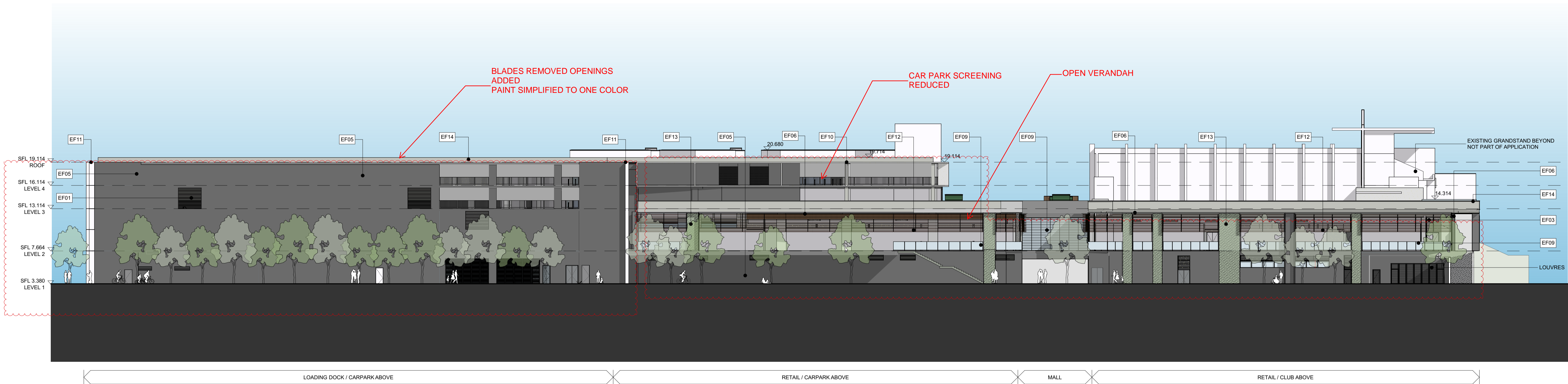
1 ELEVATION WOOLLOOWARE BAY ELEVATION (NORTH) 1:250
