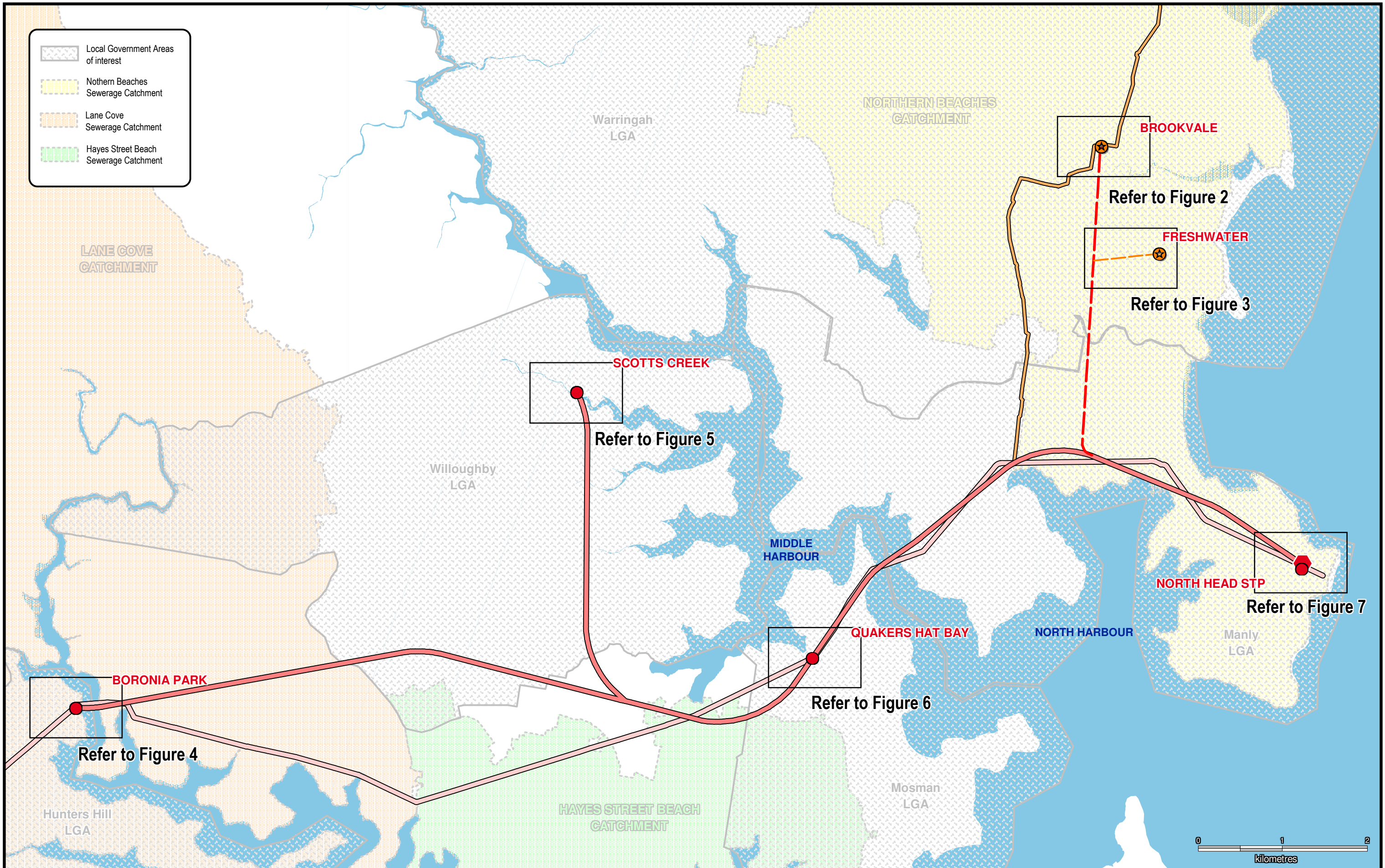
Figure 1: Northern Suburbs Sewage Treatment System
