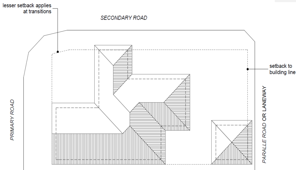
Figure 2.2.5.2 Frontage setbacks for corner lots
