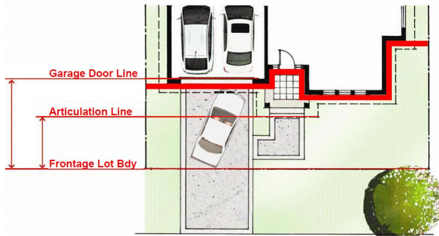
Figure 3.1.3.4: Example of diagonal driveway car parking space in double width driveway with 4.5m setback to garage door line. = Frontage Building Line
