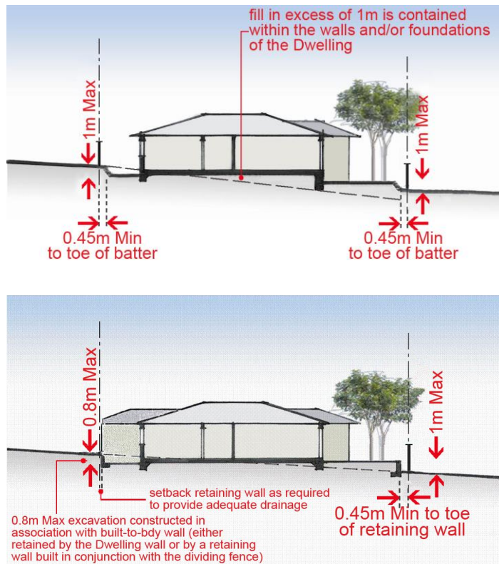
Figure 2.2.18.1 Retaining Walls and unprotected embankments
