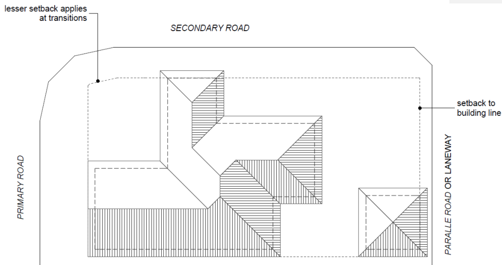
Figure 3.1.2.1 Frontage Setbacks for Corner Lots
