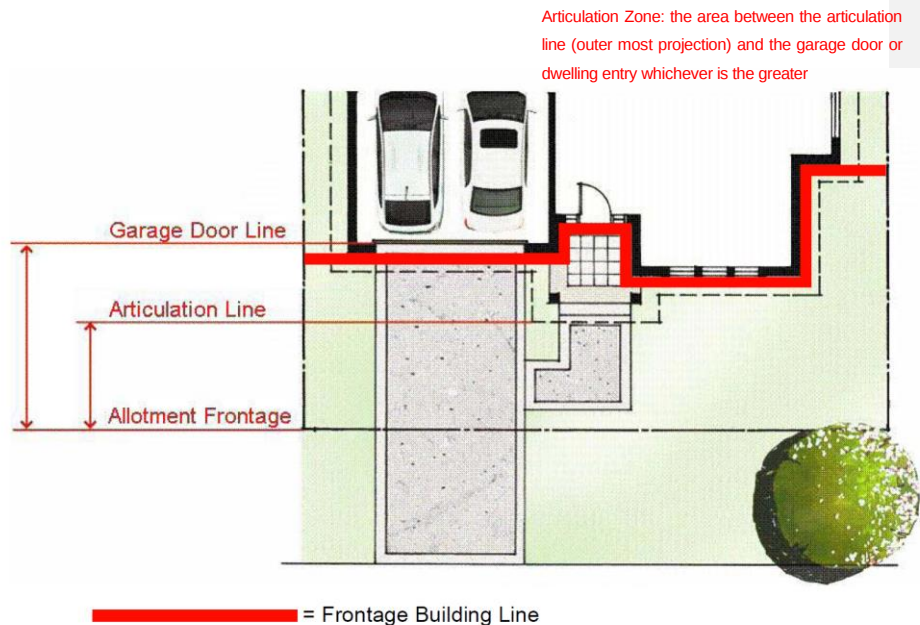
Figure 2.2.5.1 Frontage Setback Terminology
