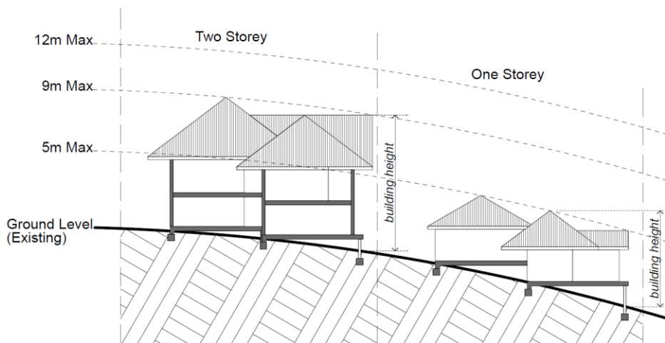
Figure 2.2.4.1 Overall Building Height
