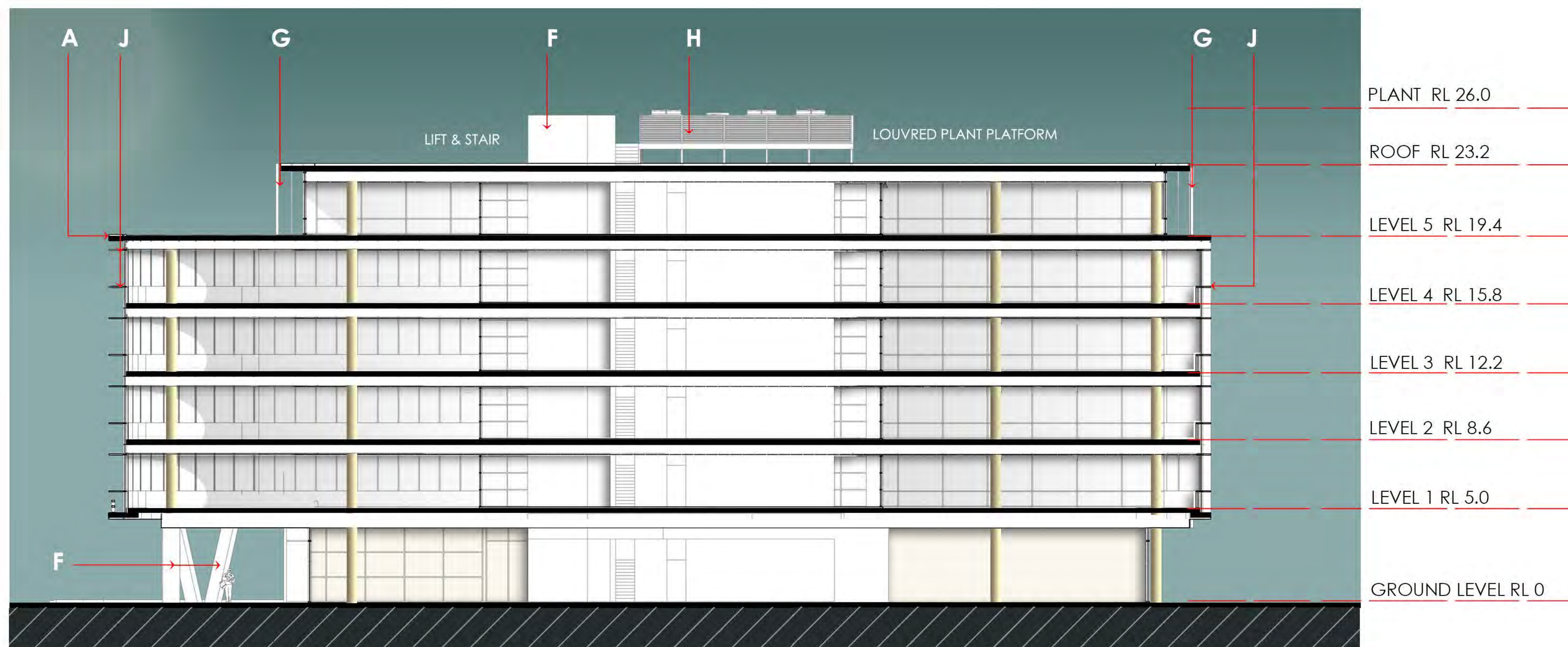
SECTION BB
