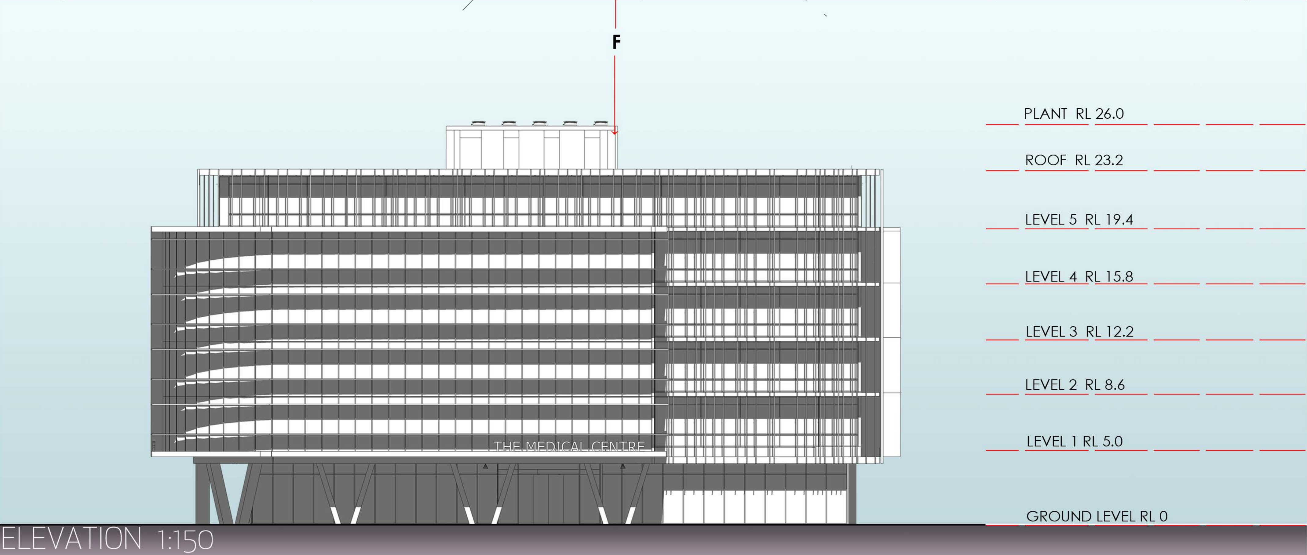
ELEVATION VIEW NTS
