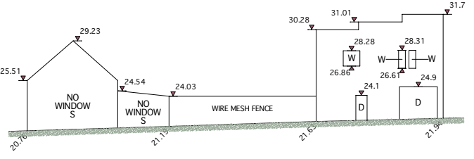
SOUTHERN ELEVATION No. 50 EVELEIGH STREET & No. 2 HOLDEN STREET
