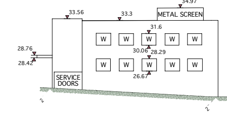
EASTERN ELEVATION COMMUNITY CENTRE LOUISE STREET
