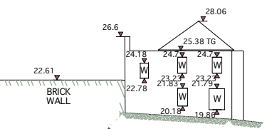
EASTERN ELEVATION No. 13 VINE STREET
