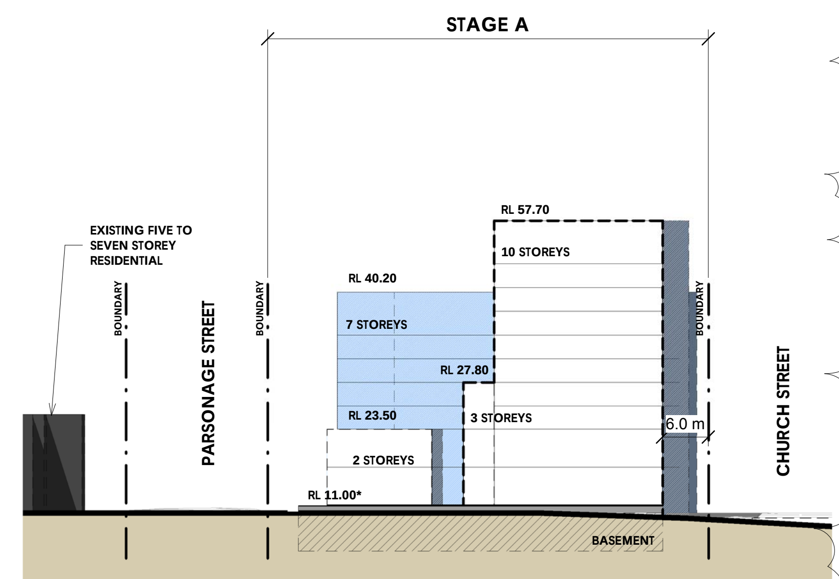
A. Elevation 3 FIGURE 18 REV 12 1 : 500
