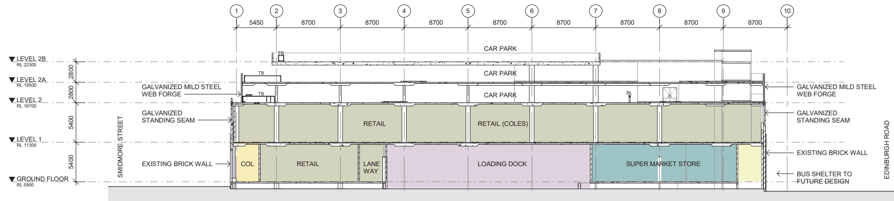
4 SECTION NORTH/SOUTH 1 : 250
