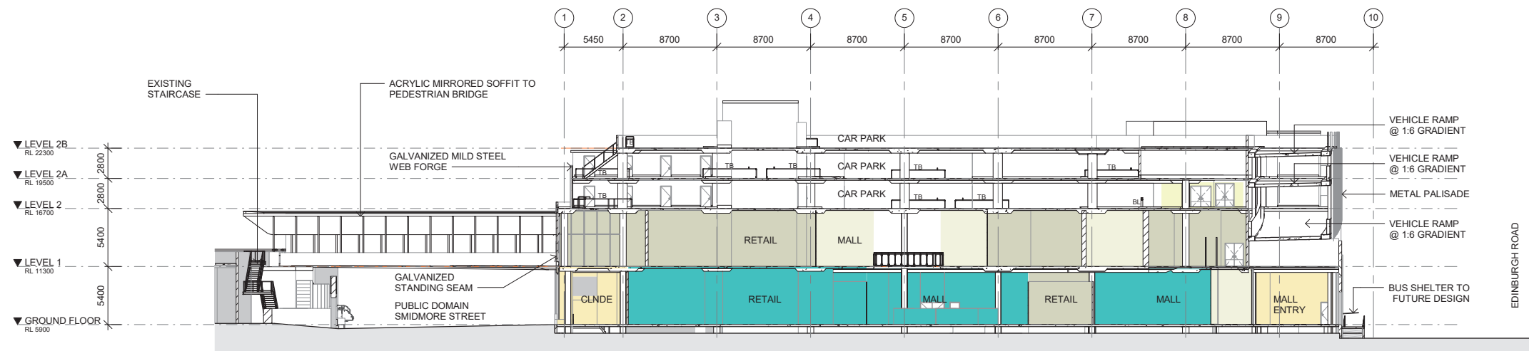
3 SECTION NORTH / SOUTH 1 : 250
