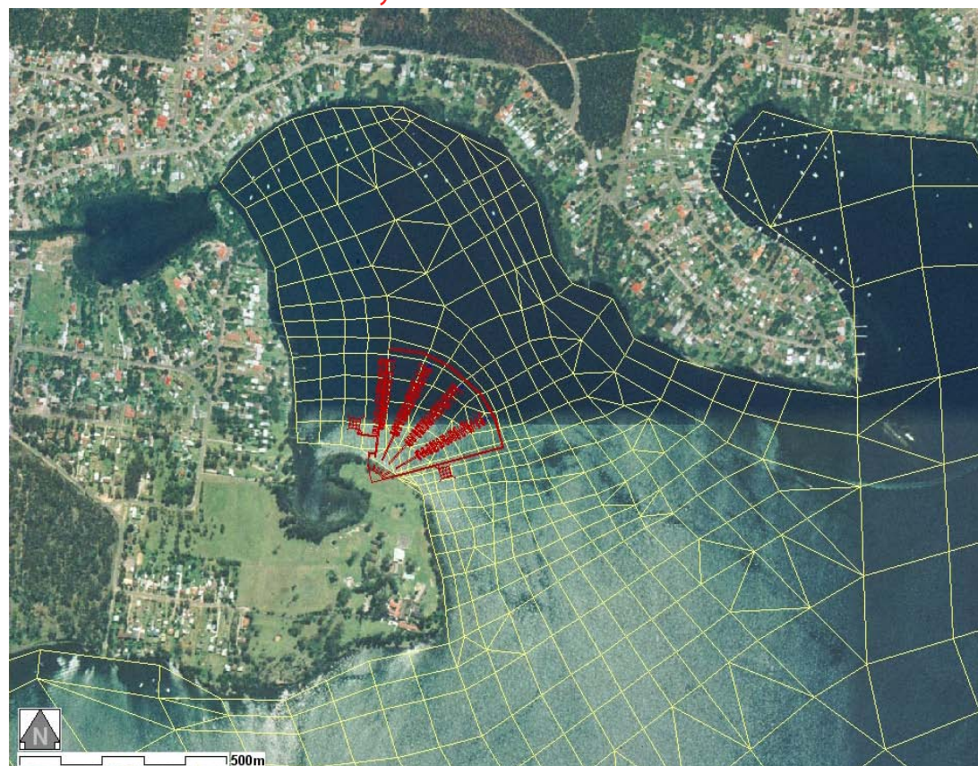
RMA Model Mesh - Bonnells Bay Area
